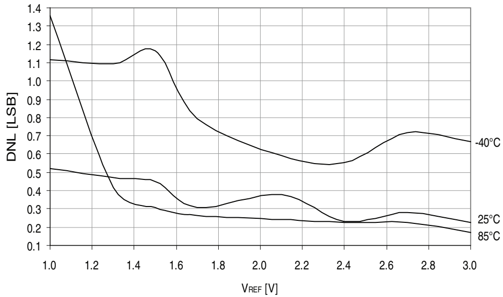
Figure 38-49. DNL error vs. V_{REF} . T = 25^{\circ}\text{C} , V_{CC} = 3.6\text{V} .
