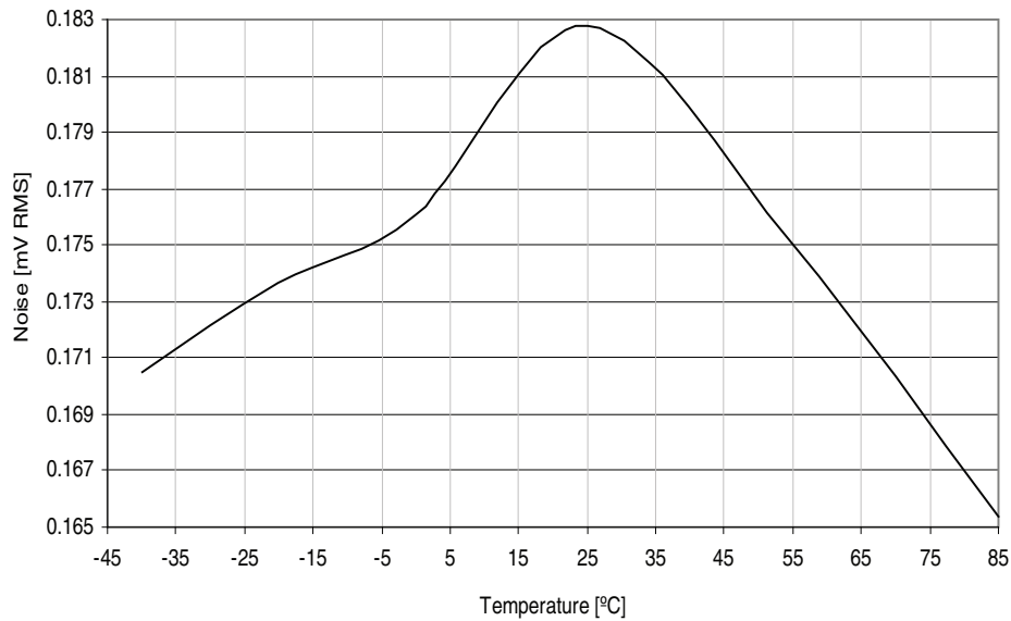
Figure 38-50. DAC noise vs. temperature. V_{CC} = 3.0\text{V} , V_{REF} = 2.4\text{V} .
