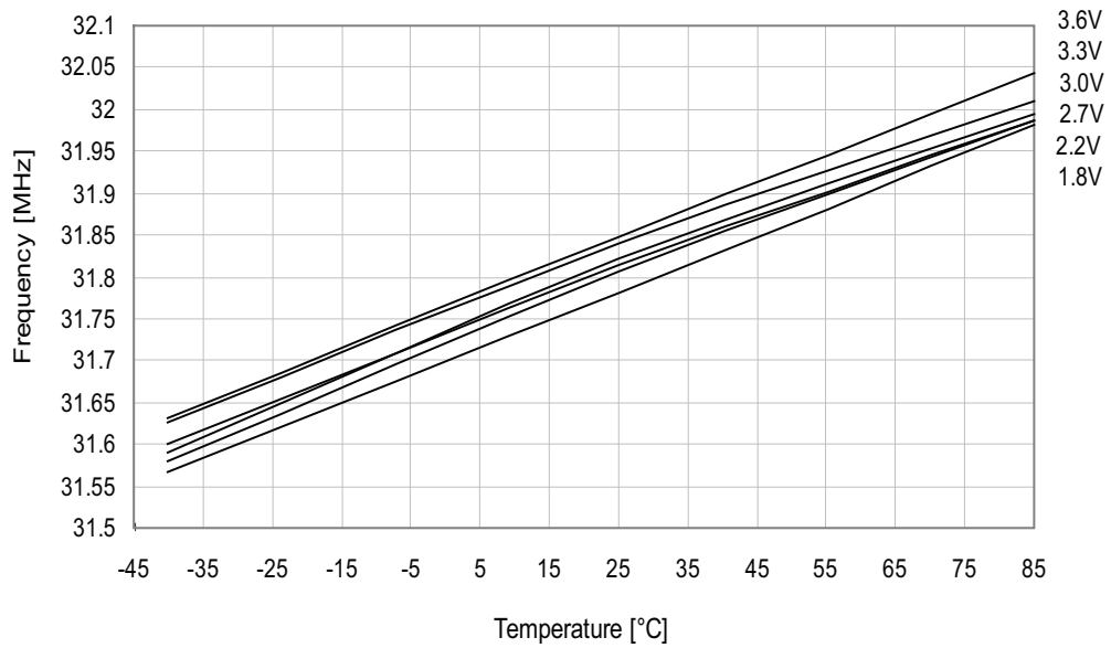
Figure 34-151. 32MHz internal oscillator frequency vs. temperature. DFLL enabled, from the 32.768kHz internal oscillator.
