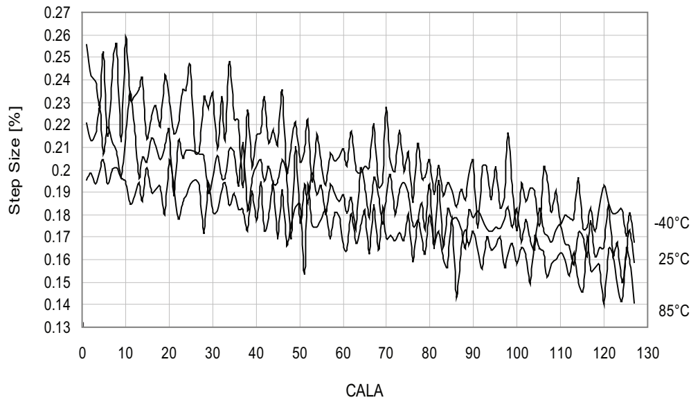
Figure 34-76. 48MHz internal oscillator CALA calibration step size.
