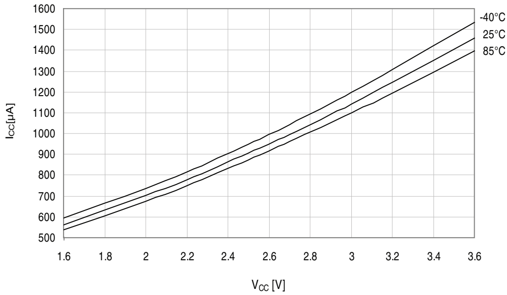
Figure 34-93. Idle mode current vs. V_{CC} .
