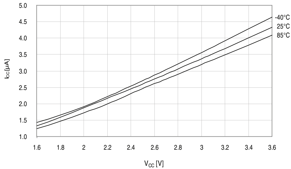
Figure 34-85. Active mode supply current vs. V_{CC} .
