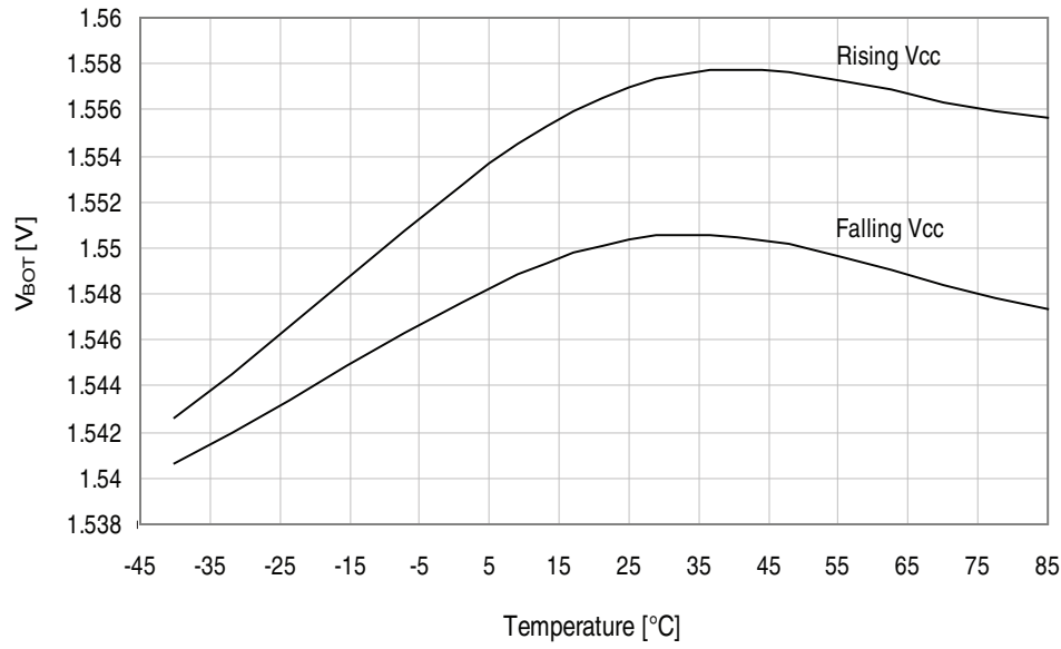
Figure 34-56. BOD thresholds vs. temperature.
