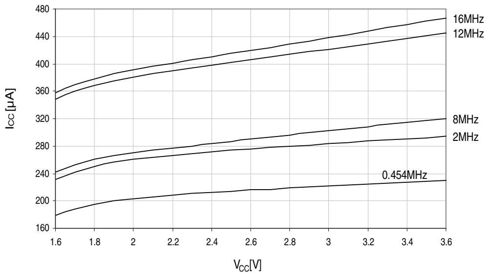
Figure 34-99. Standby supply current vs. V_{CC} . 25°C, running from different crystal oscillators.
