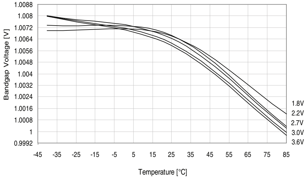
Figure 34-133. ADC Internal 1.0V reference vs. temperature.
