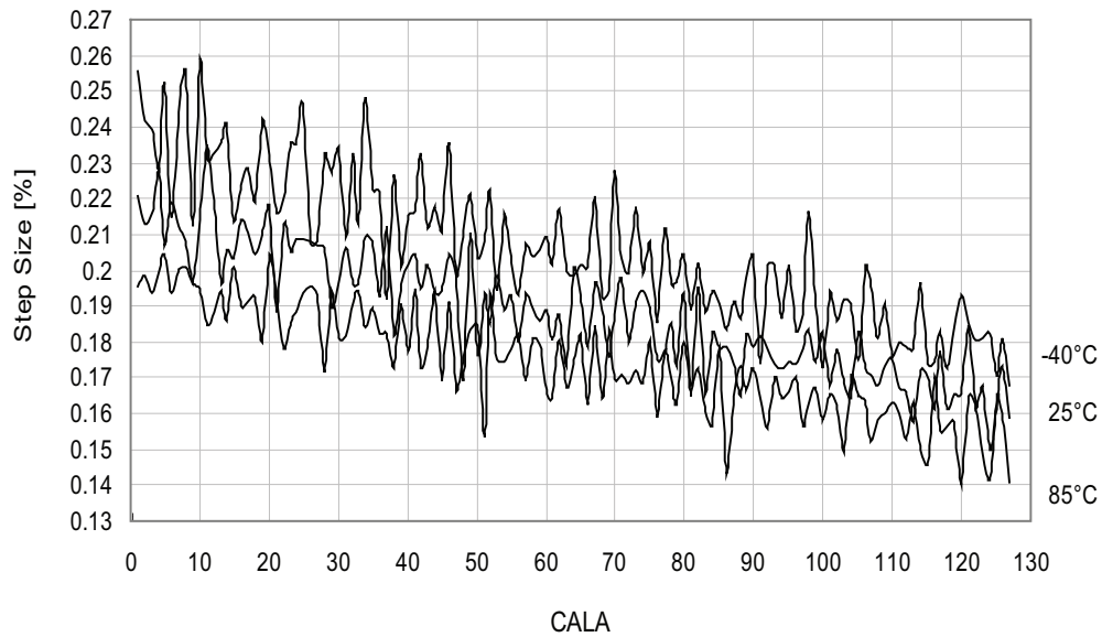
Figure 34-155. 48MHz internal oscillator CALA calibration step size.
