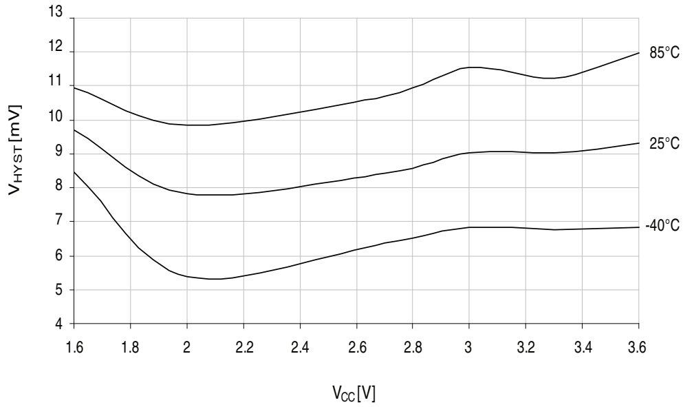
Figure 34-127. Analog comparator hysteresis vs. V_{CC} . High speed, large hysteresis.
