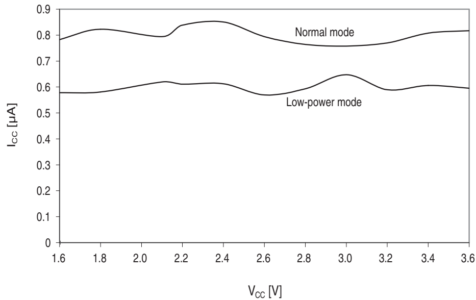
Figure 34-97. Power-save mode supply current vs. V CC .
