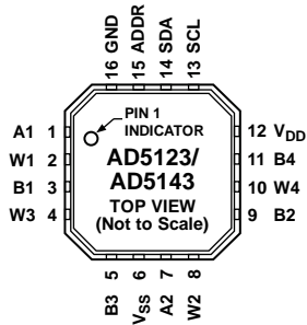
Figure 4. Pin Configuration
