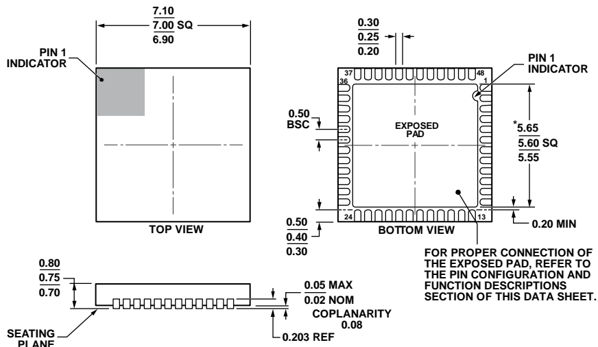
Figure 56. 48-Lead Lead Frame Chip Scale Package [LFCSP_WQ] 7 mm × 7 mm Body, Very Very Thin Quad (CP-48-13) Dimensions shown in millimeters
