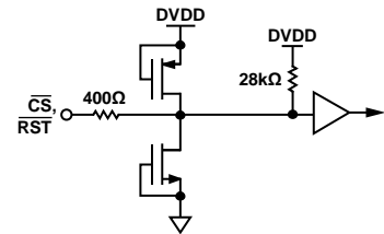
Figure 24. Equivalent CS or RST Input Circuit
