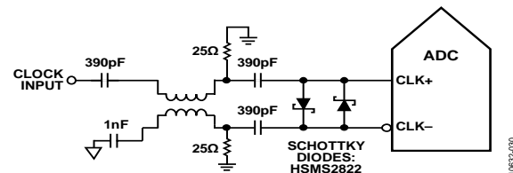
Figure 33. Balun-Coupled Differential Clock (Up to 625 MHz)
