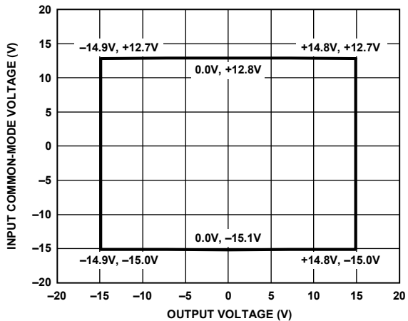
Figure 17. Input Common-Mode Voltage vs. Output Voltage, G = 100 , V_S = \pm 15V
