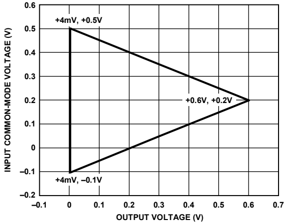
Figure 16. Input Common-Mode Voltage vs. Output Voltage, G = 1 , V_S = 2.7V
