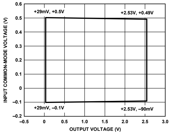
Figure 20. Input Common-Mode Voltage vs. Output Voltage, G = 100 , V_S = 2.7V
