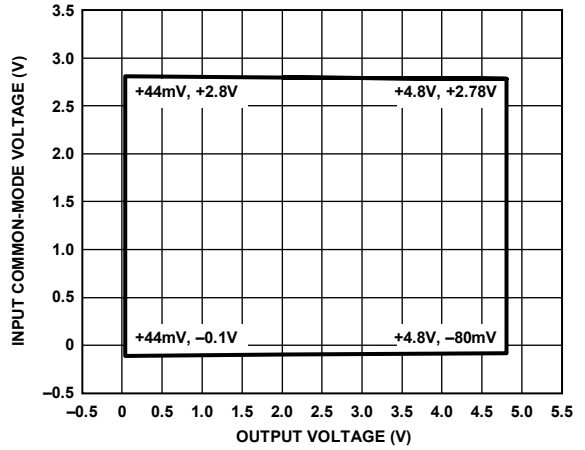
Figure 18. Input Common-Mode Voltage vs. Output Voltage, G = 100 , V_S = 5V
