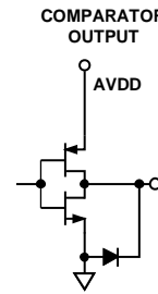
Figure 22. Comparator Outputs
