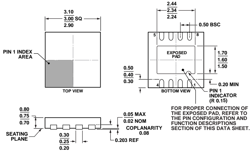
Figure 76. 8-Lead Lead Frame Chip Scale Package [LFCSF_WD] 3 mm × 3 mm Body, Very Very Thin, Dual Lead (CP-8-11) Dimensions shown in millimeters
