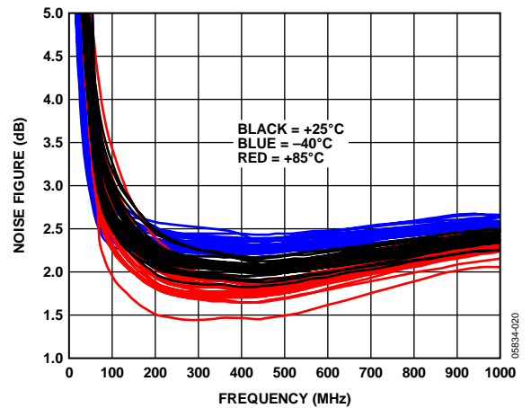
Figure 20. Noise Figure Temperature Distribution, VPOS = 3 V
