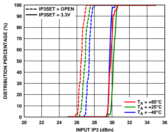
Figure 29. Input IP3
