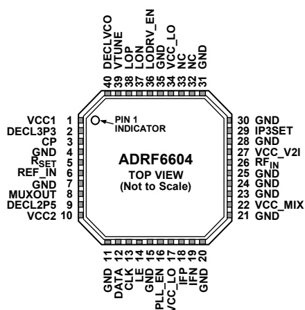
Figure 3. Pin Configuration
