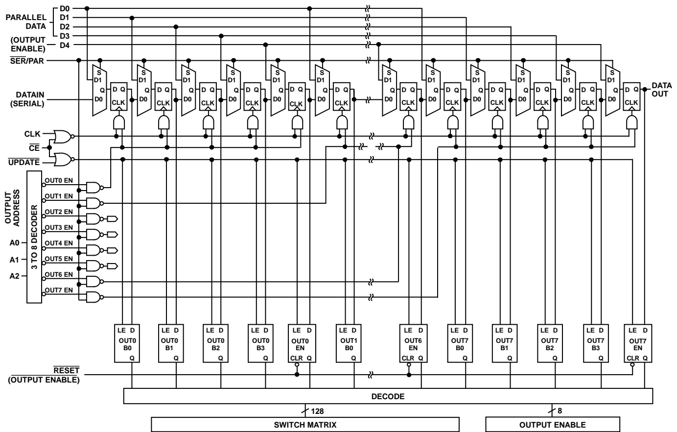
Figure 6. Logic Diagram
