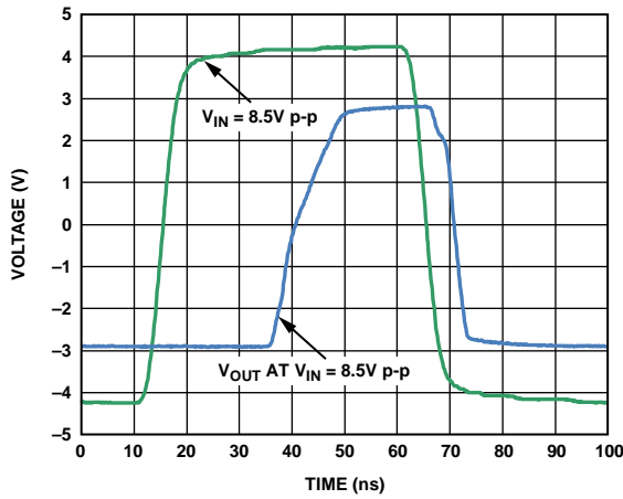
Figure 50. ADV3224 Overdrive Recovery
