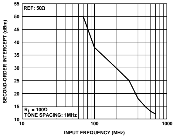
Figure 55. ADV3225 Output Second-Order Intercept, 100 \Omega Load
