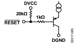
Figure 63. Reset Input
