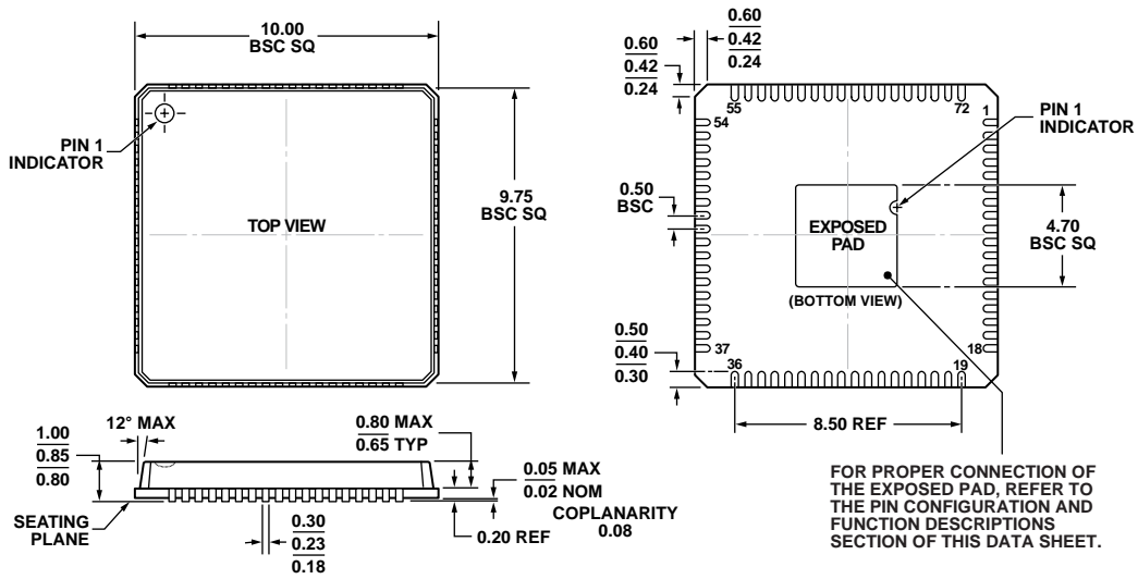
Figure 66. 72-Lead Lead Frame Chip Scale Package [LFCSP_VQ] 10 mm × 10 mm Body, Very Thin Quad (CP-72-1)
