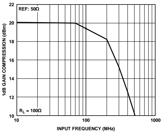
Figure 51. ADV3225 1 dB Gain Compression, 100 Ω Load
