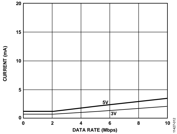
Figure 12. Typical ADuM3301W V_{DD2} Supply Current vs. Data Rate for 5 V and 3 V Operation
