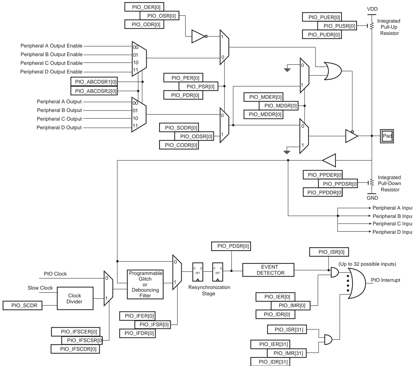
Figure 33-3. I/O Line Control Logic
