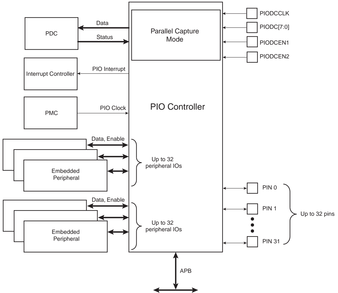
Figure 33-1. Block Diagram
