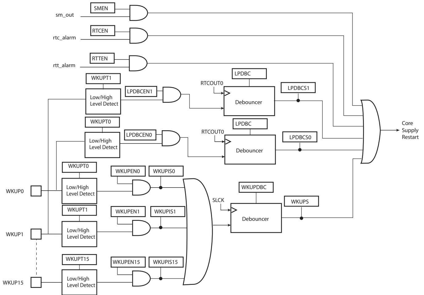
Figure 20-4. Wake-up Sources
