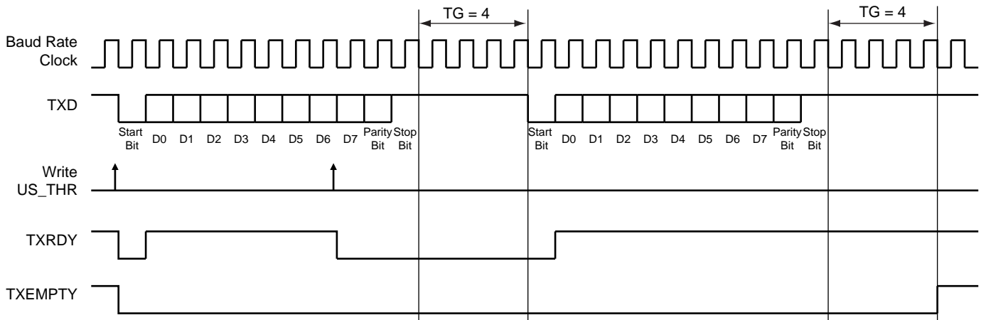
Figure 37-23. Timeguard Operations
