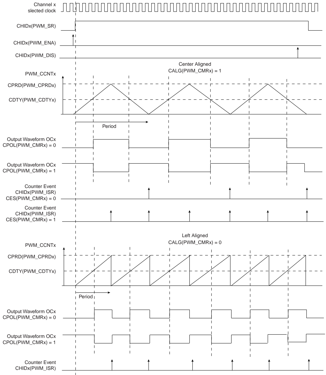
Figure 40-5. Waveform Properties
