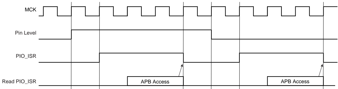
Figure 33-8. Input Change Interrupt Timings if there are no Additional Interrupt Modes
