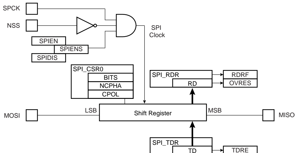
Figure 34-12. Slave Mode Functional Bloc Diagram
