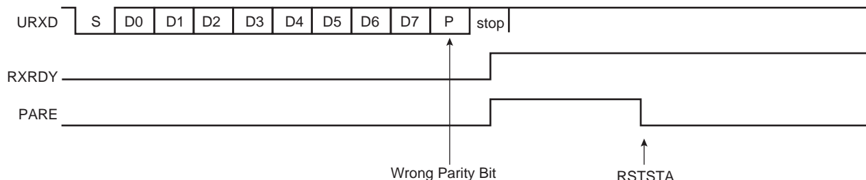
Figure 36-7. Parity Error
