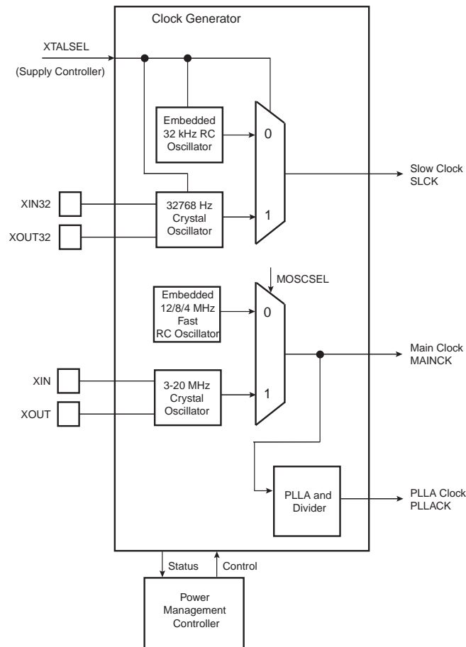
Figure 11-2. Clock Generator Block Diagram
