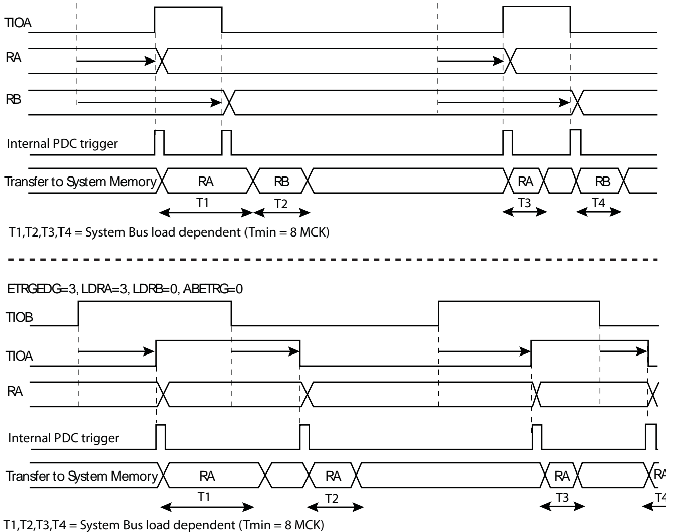
Figure 38-5. Example of transfer with PDC
