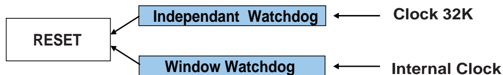
Figure 11-4. Dual Watchdog
