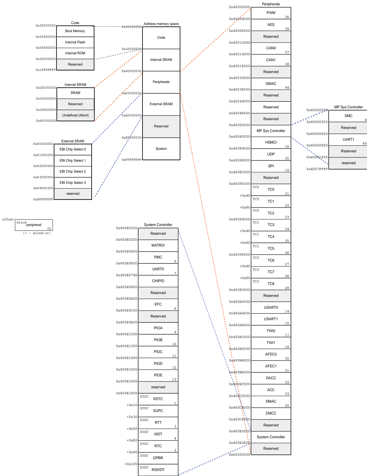
Figure 9-1. SAM4E Product Mapping
