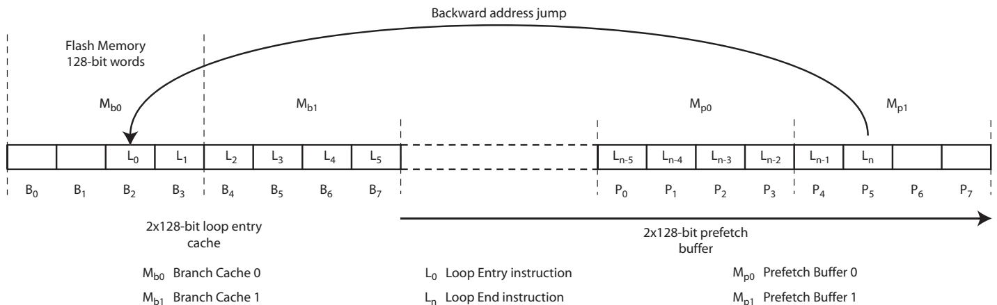
Figure 22-4. Code Loops Optimization
