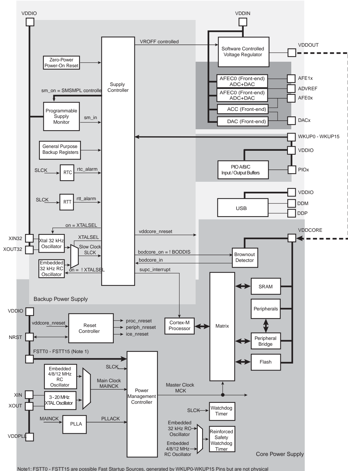
Figure 11-1. System Controller Block Diagram
