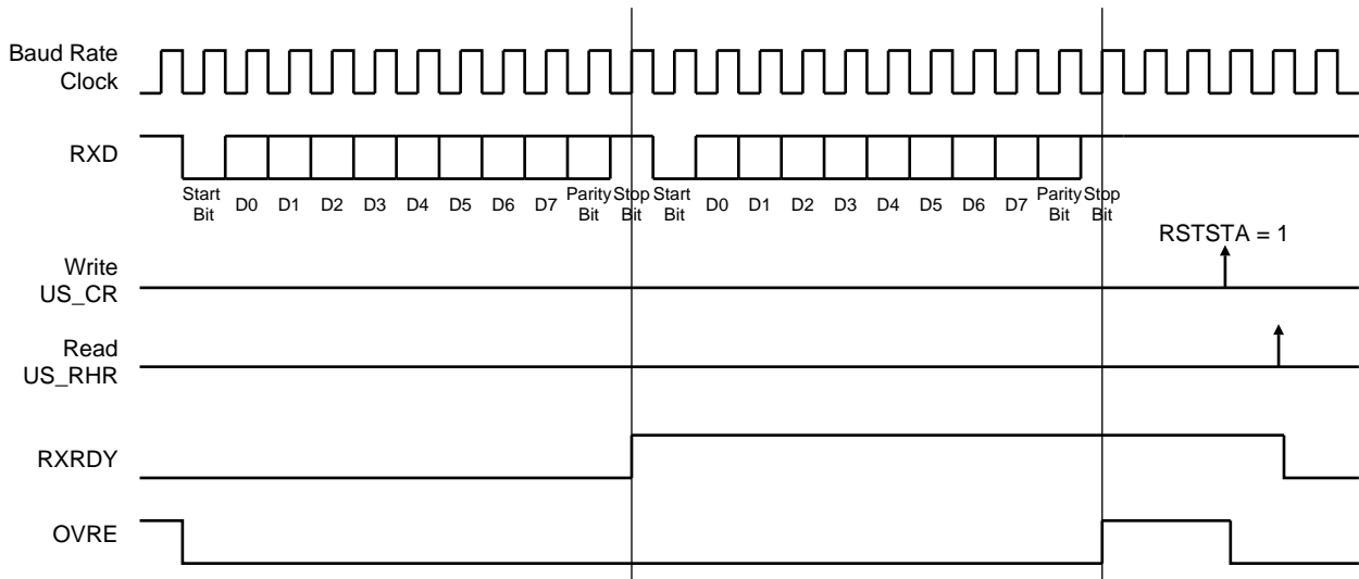
Figure 37-21. Receiver Status
