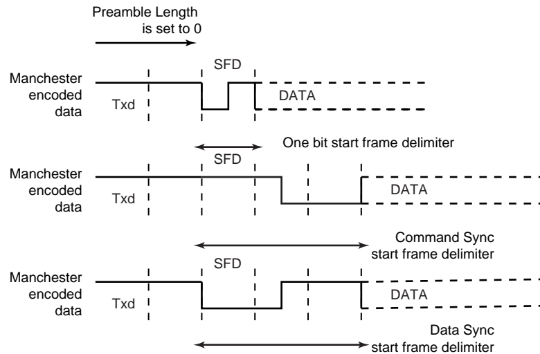
Figure 37-10. Start Frame Delimiter
