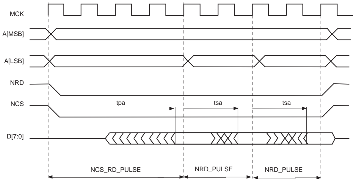
Figure 28-31. Page Mode Read Protocol (Address MSB and LSB are defined in Table 28-5 )
