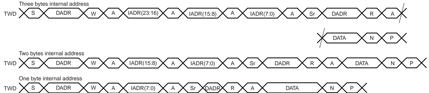
Figure 35-13. Master Read with One, Two or Three Bytes Internal Address and One Data Byte
