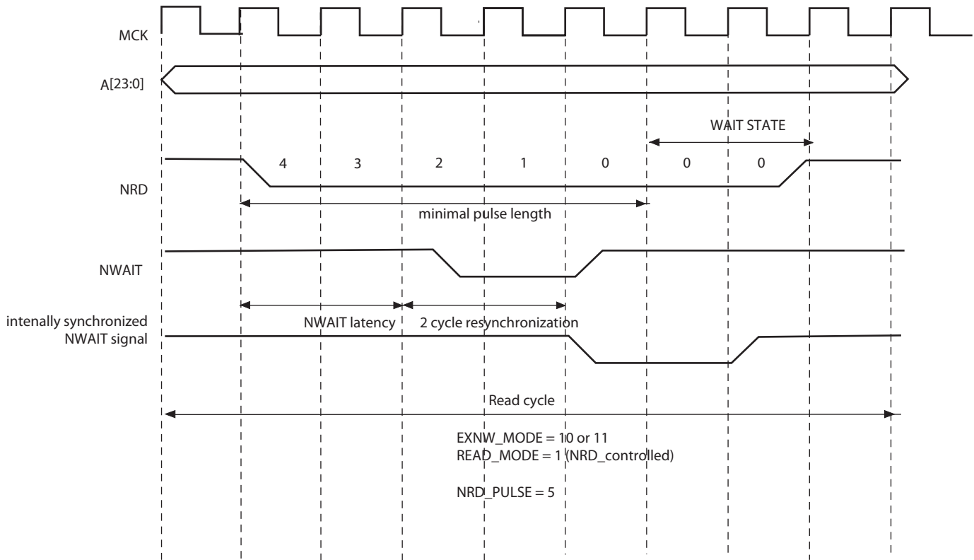
Figure 28-27. NWAIT Latency
