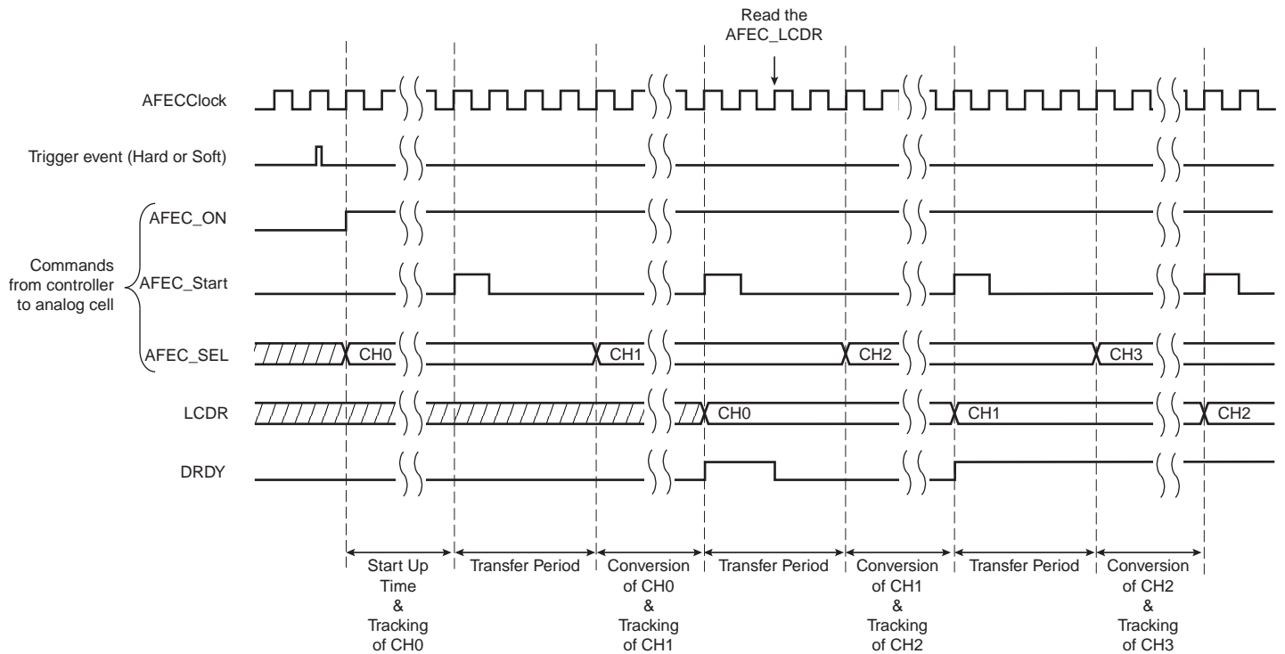
Figure 43-3. Sequence of AFEC conversions when Tracking time < Conversion time
