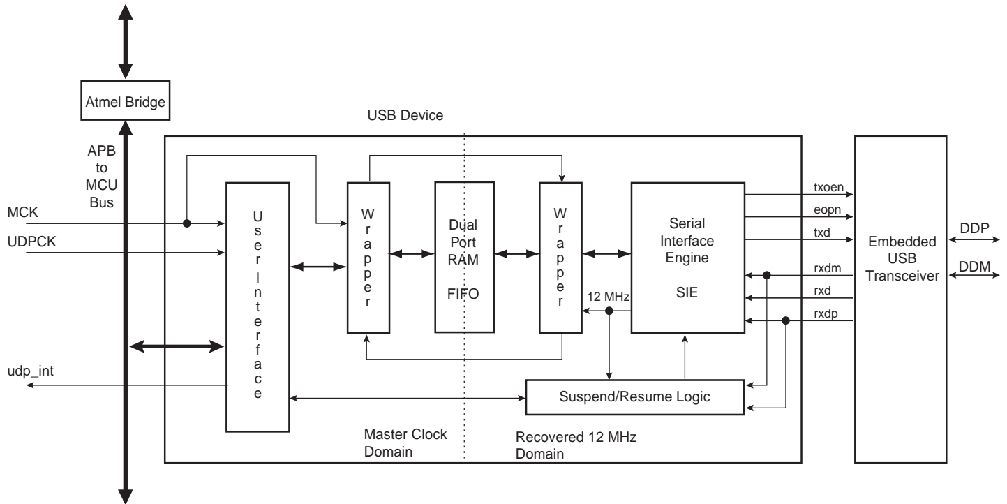
Figure 41-1. Block Diagram
