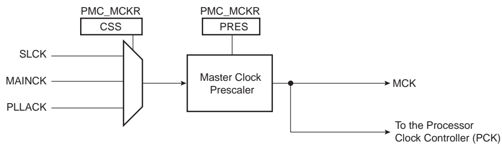
Figure 30-6. Master Clock Controller
