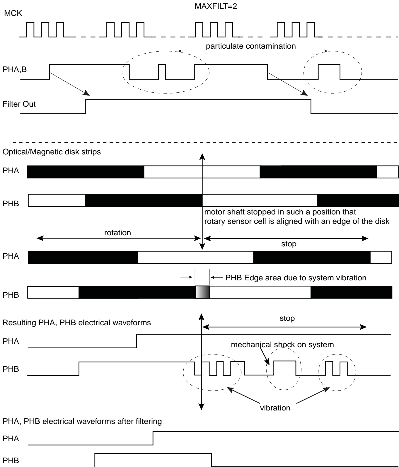
Figure 38-19. Filtering Examples
