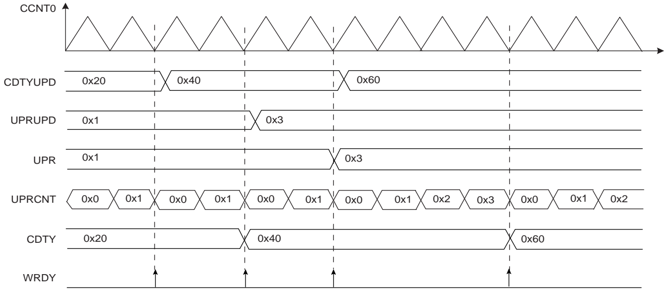
Figure 40-13. Method 2 (UPDM=1)
