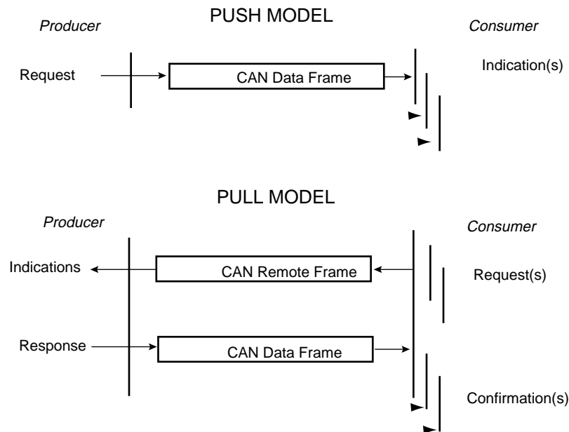
Figure 32-16.Producer / Consumer Model
