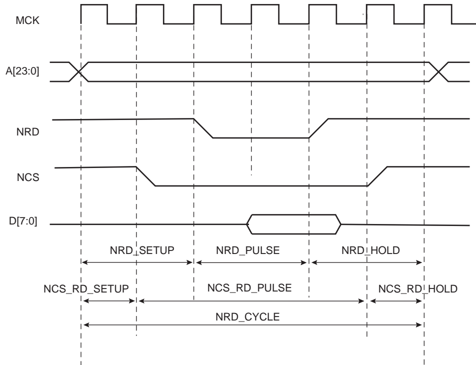
Figure 28-5. Standard Read Cycle
