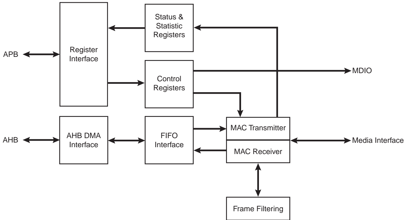
Figure 44-1. Block Diagram
