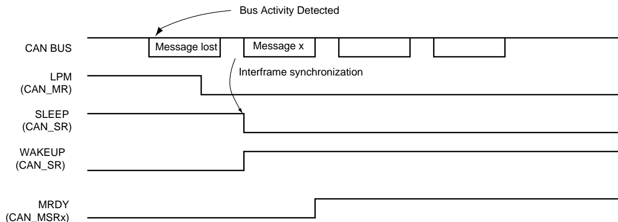
Figure 32-9. Disabling Low-power Mode
