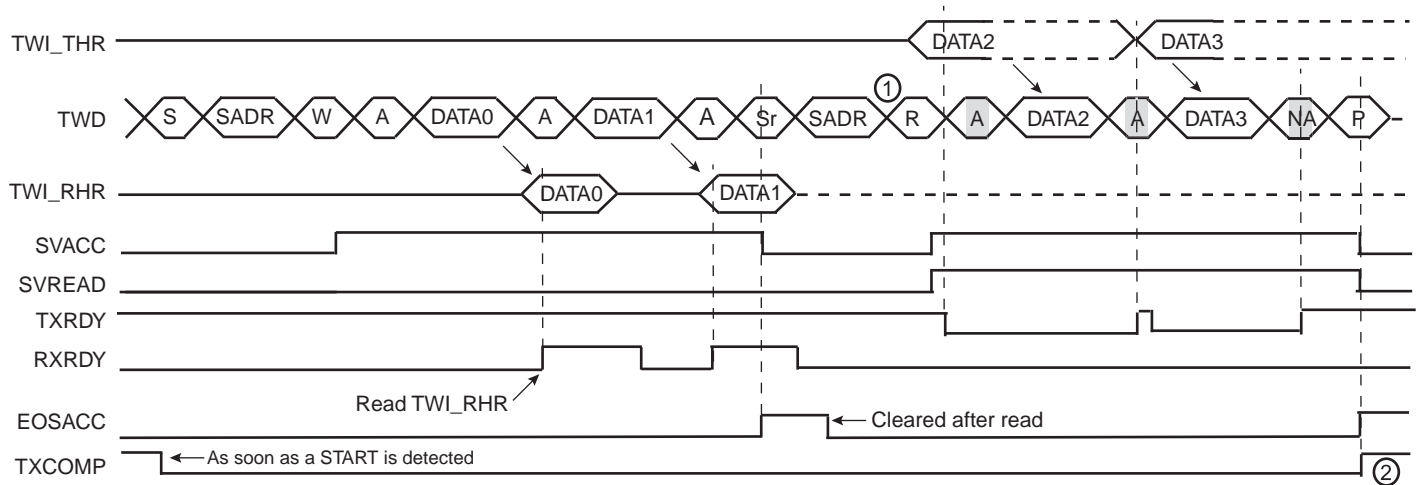
Figure 35-32. Repeated Start + Reversal from Write to Read Mode
