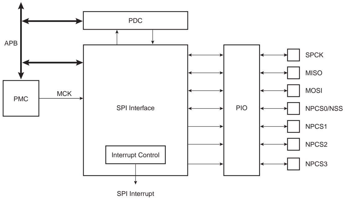
Figure 34-1. Block Diagram
