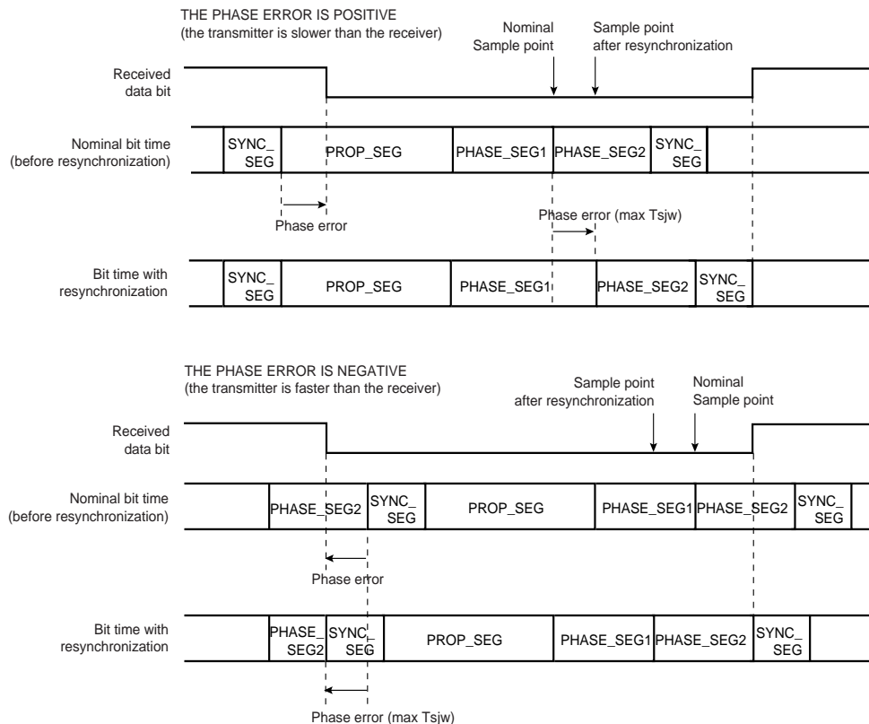
Figure 32-6. CAN Resynchronization
