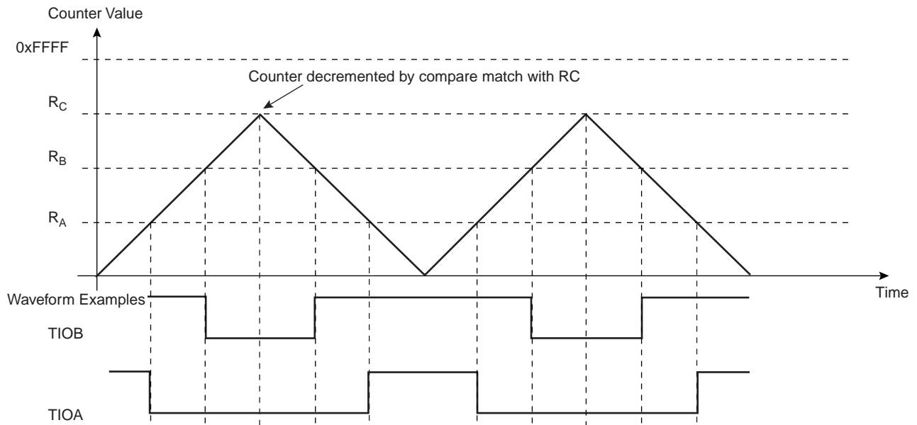
Figure 38-14. WAVSEL = 11 Without Trigger
