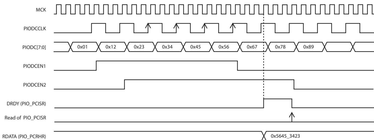
Figure 33-11. Parallel Capture Mode Waveforms (DSIZE = 2, ALWAYS = 0, HALFS = 0)
