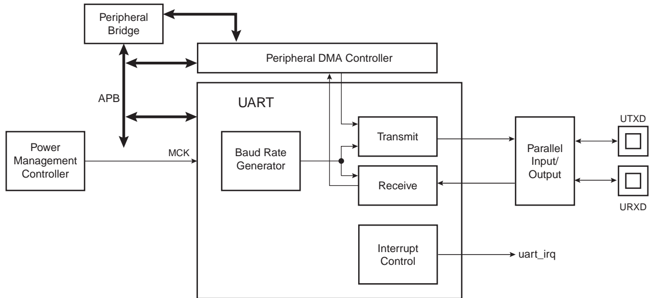
Figure 36-1. UART Functional Block Diagram
