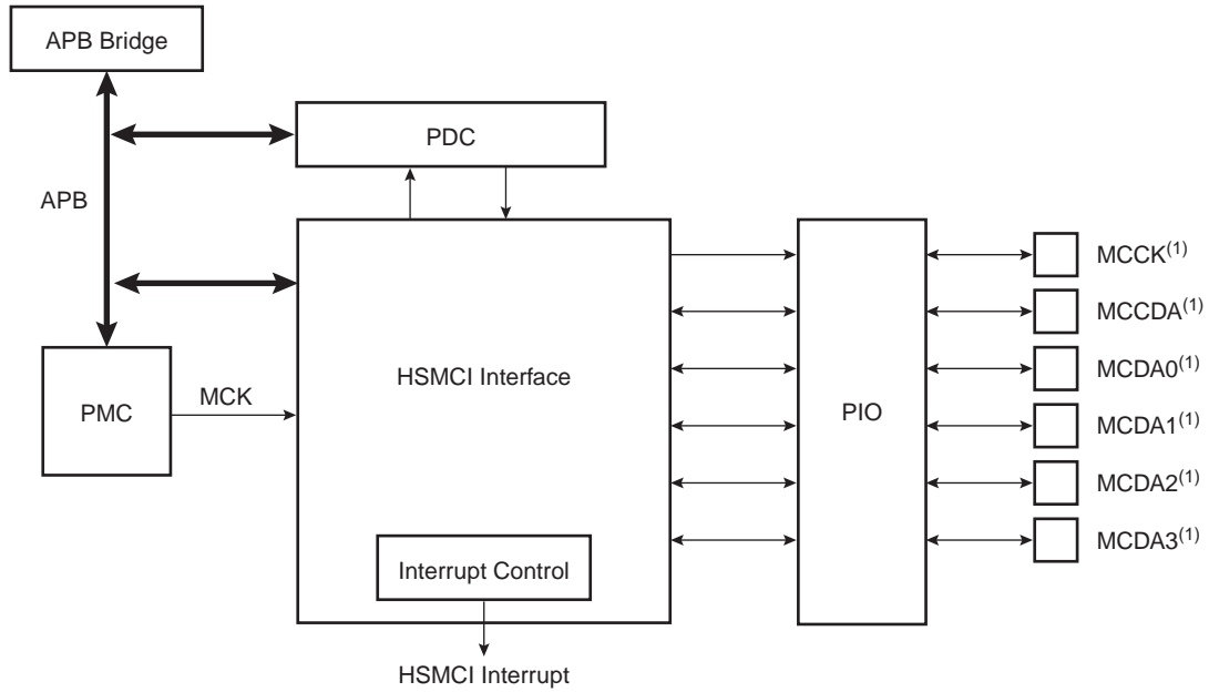
Figure 39-1. Block Diagram
