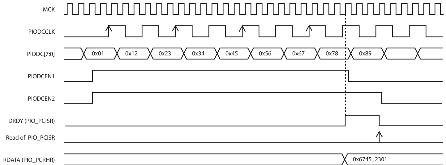
Figure 33-13. Parallel Capture Mode Waveforms (DSIZE=2, ALWYS=0, HALFS=1, FRSTS=0)
