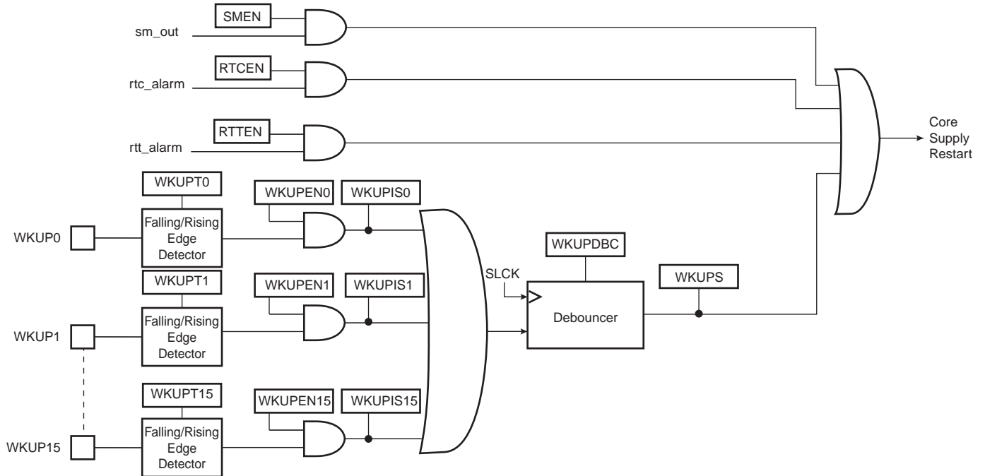
Figure 5-3. Wake-up Source
