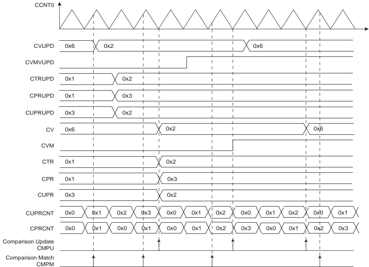
Figure 40-17. Comparison Waveform
