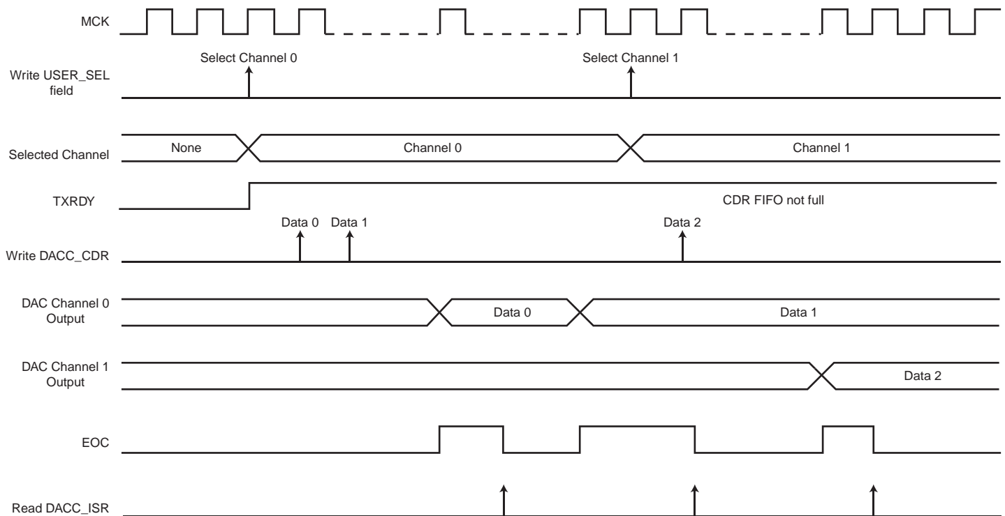
Figure 45-2. Conversion Sequence
