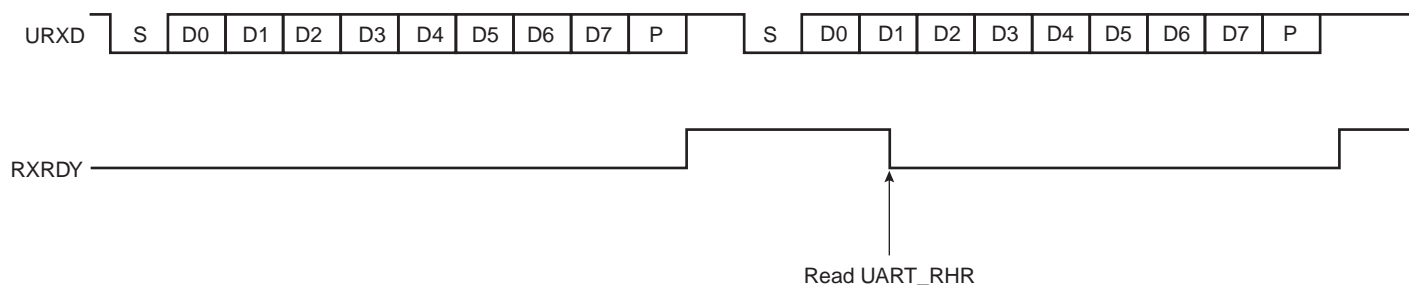
Figure 36-5. Receiver Ready
