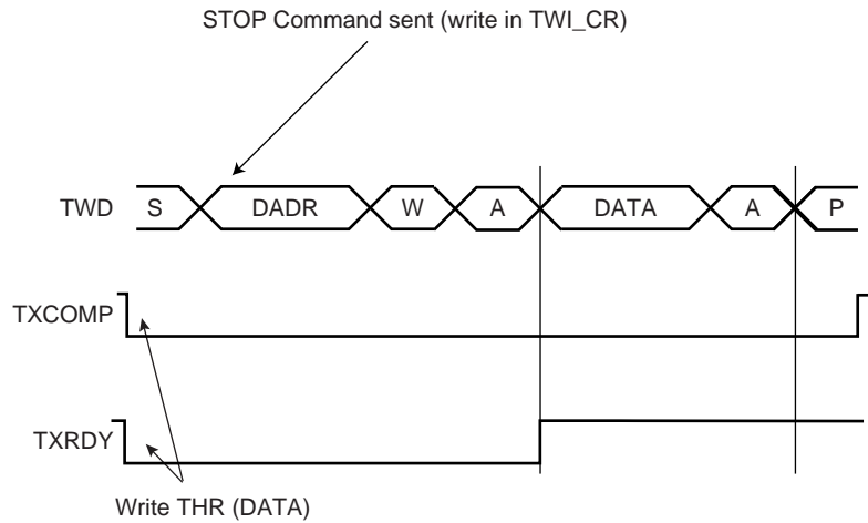
Figure 35-6. Master Write with One Data Byte
