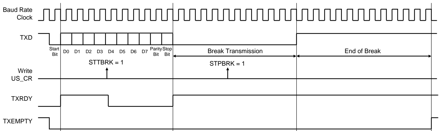
Figure 37-26. Break Transmission
