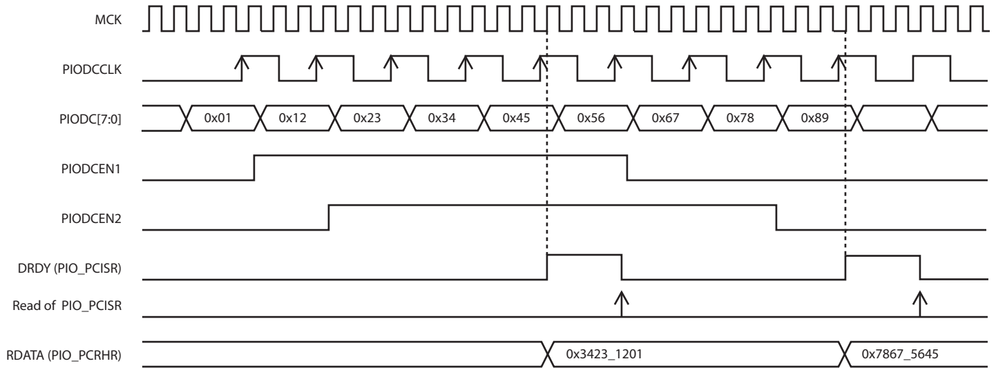
Figure 33-12. Parallel Capture Mode Waveforms (DSIZE=2, ALWYS=1, HALFS=0)
