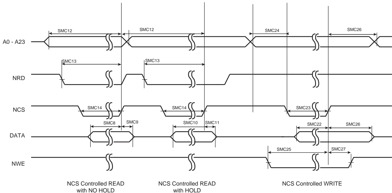
Figure 46-20. SMC Timings - NCS Controlled Read and Write
