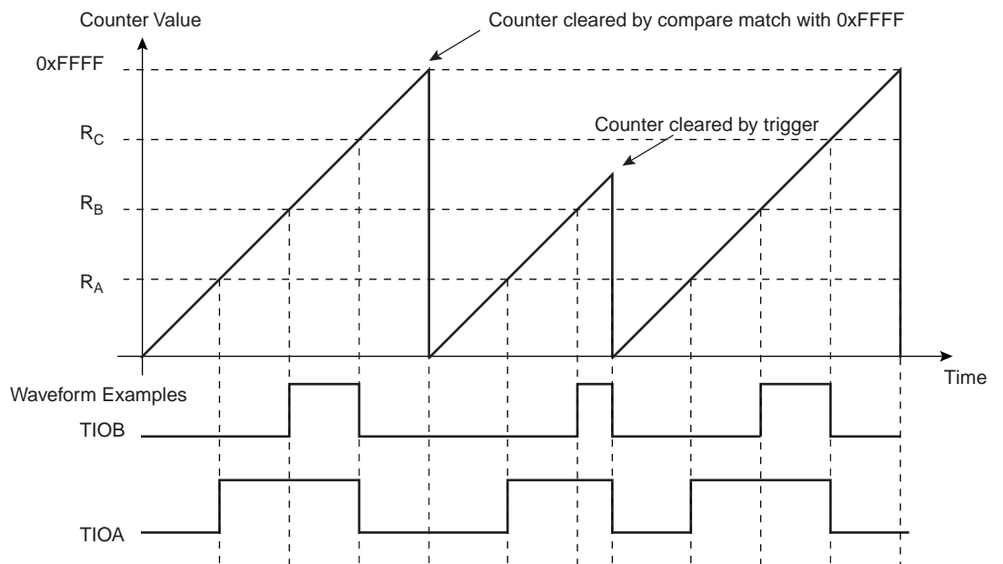
Figure 38-9. WAVSEL= 00 with trigger
