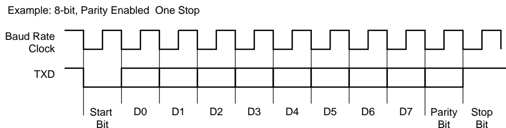
Figure 37-6. Character Transmit
