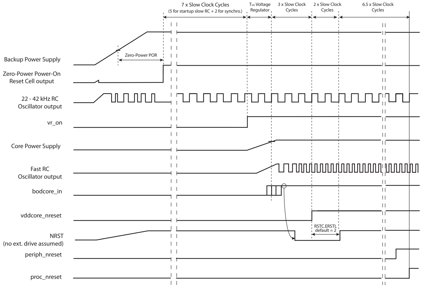
Figure 20-3. Raising the VDDIO Power Supply
