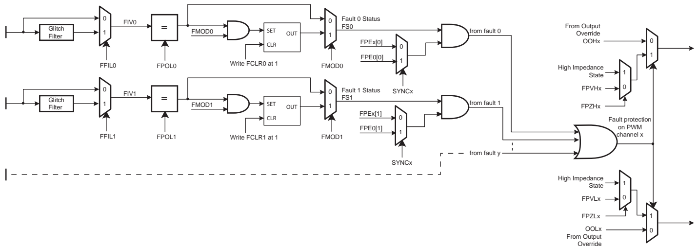
Figure 40-9. Fault Protection
