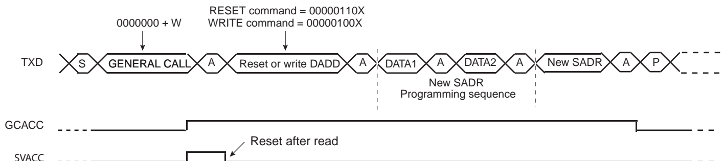
Figure 35-28. Master Performs a General Call
