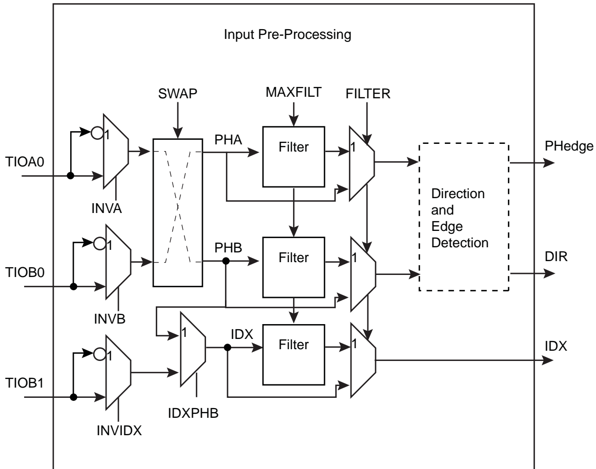
Figure 38-18. Input Stage
