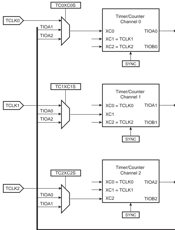
Figure 38-2. Clock Chaining Selection
