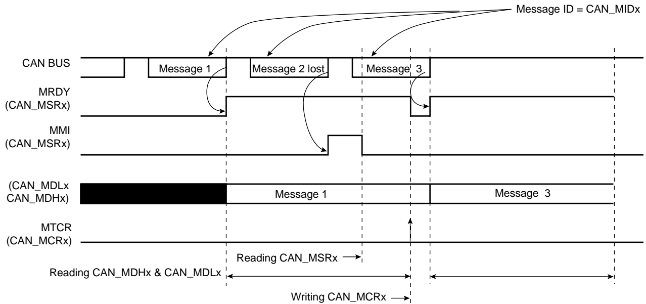
Figure 32-11. Receive Mailbox
