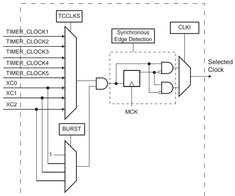
Figure 38-3. Clock Selection
