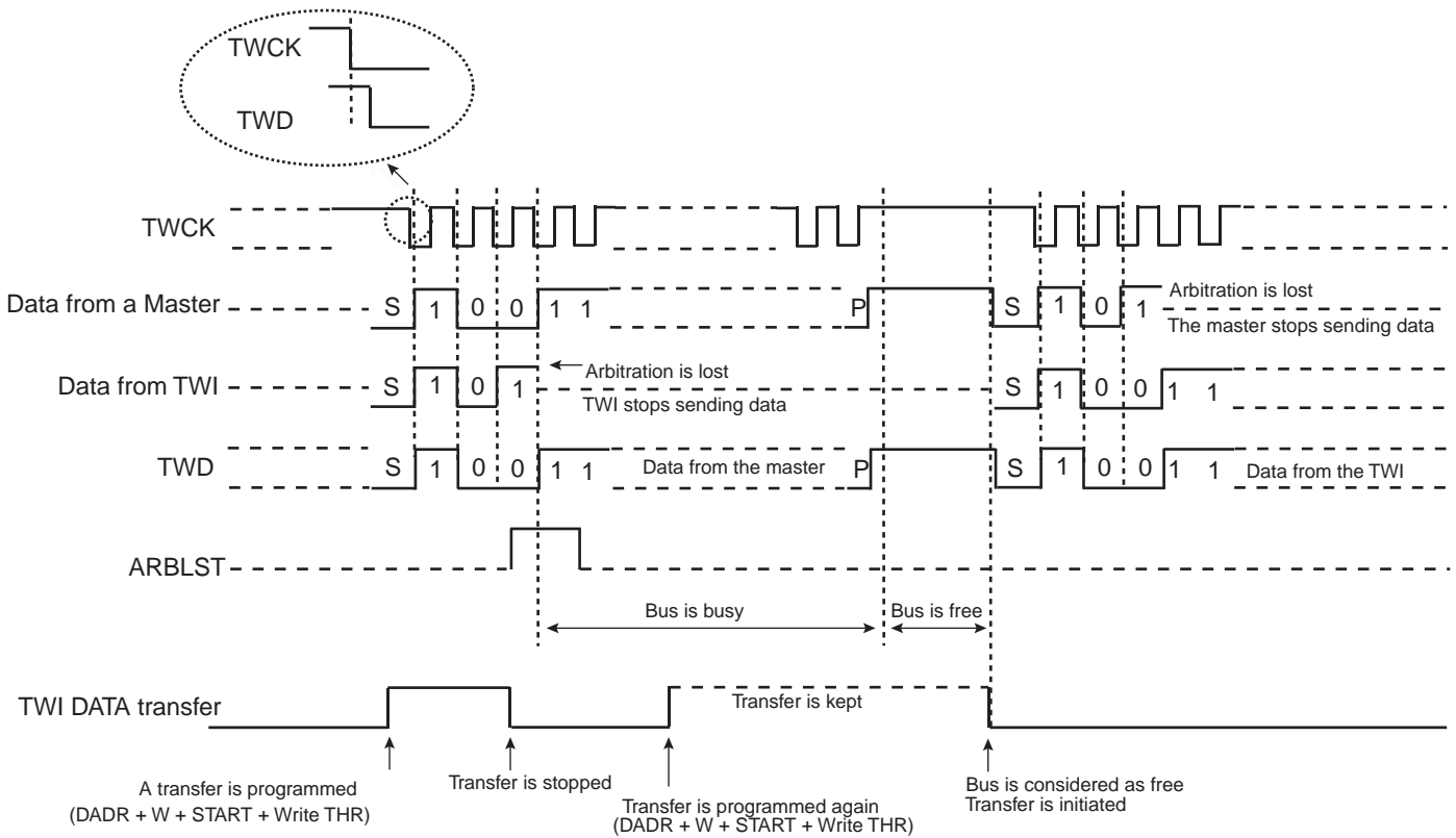
Figure 35-23. Arbitration Cases
