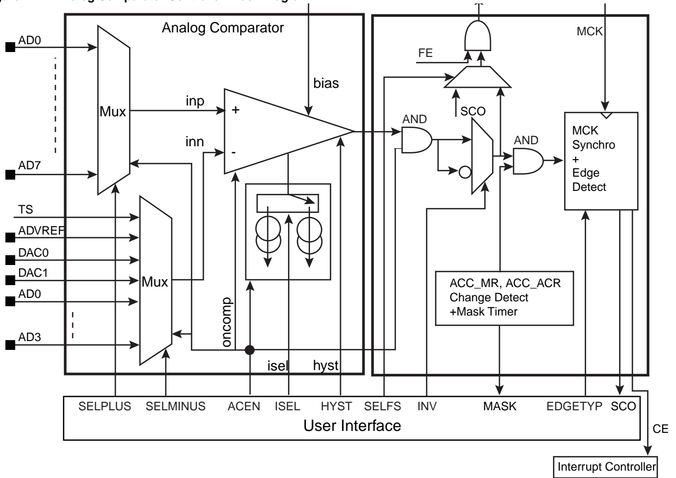
Figure 42-1. Analog Comparator Controller Block Diagram
