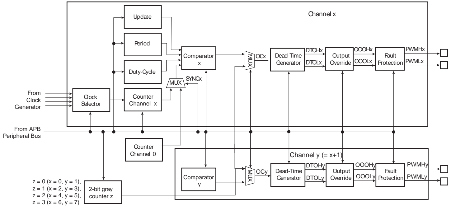
Figure 40-3. Functional View of the Channel Block Diagram
