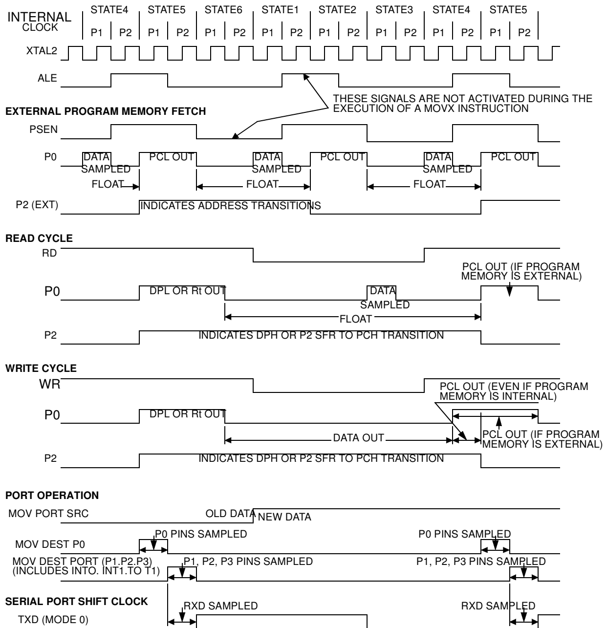
Figure 45. Clock Waveforms
