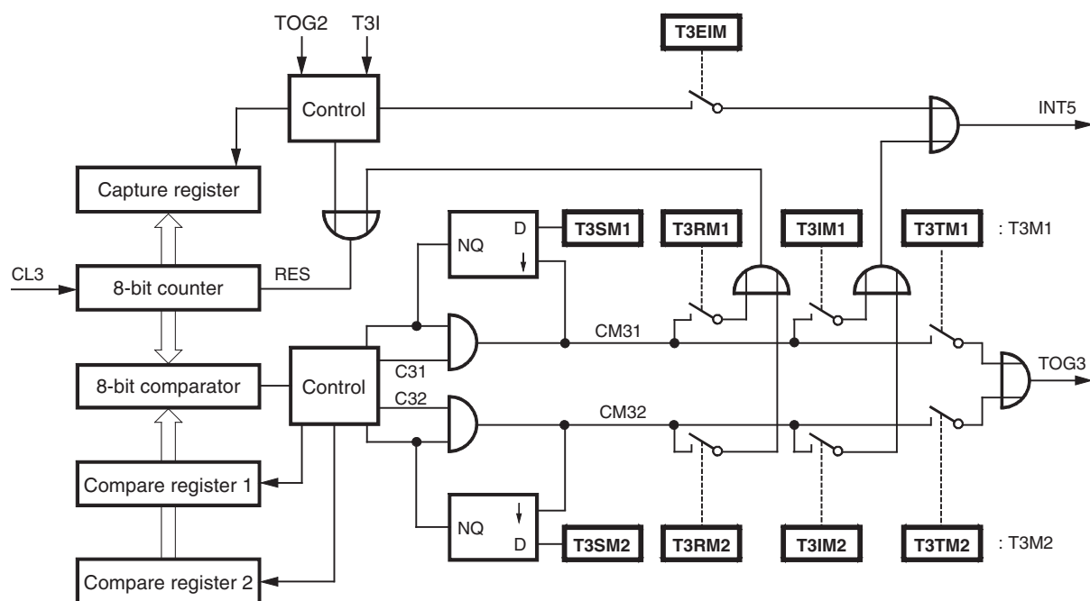
Figure 23-2. Counter 3 Stage
