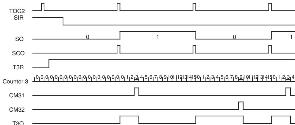
Figure 23-9. Pulse-width Modulation
