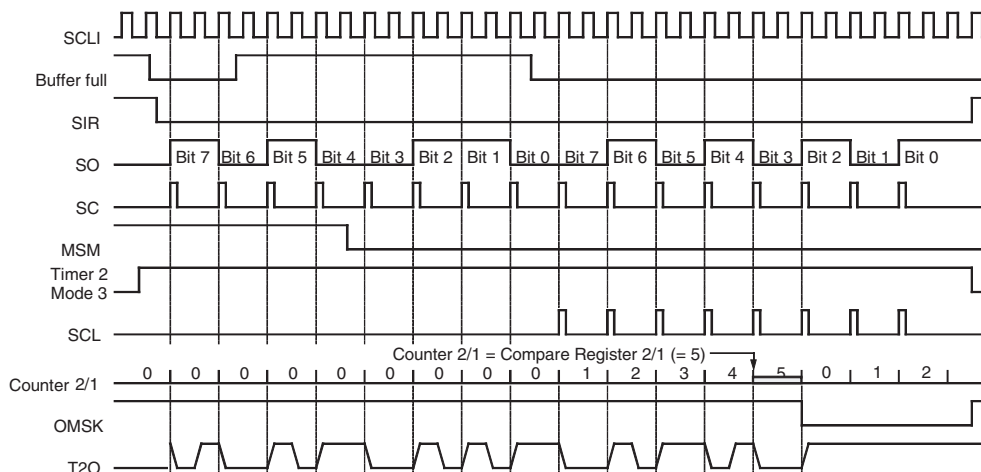
Figure 24-6. Biphase Modulation 2
