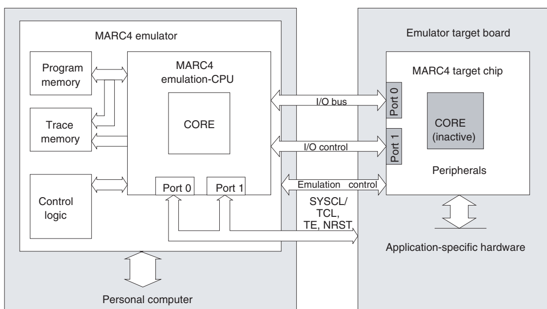
Figure 30-1. MARC4 Emulation
