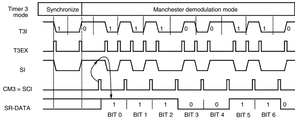
Figure 5-57. Manchester Demodulation
