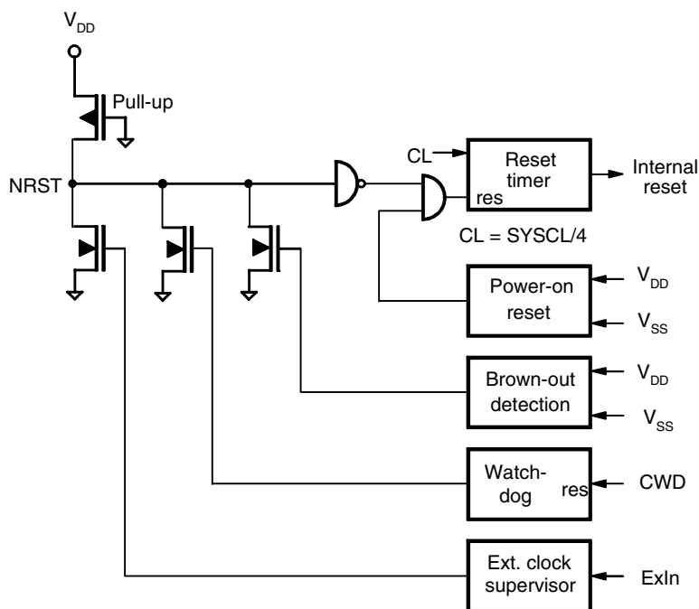
Figure 4-7. Reset Configuration
