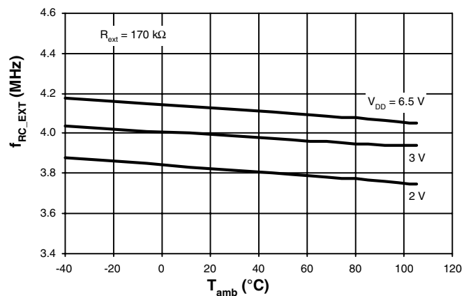
Figure 11-10. External RC Frequency versus T_{amb}
