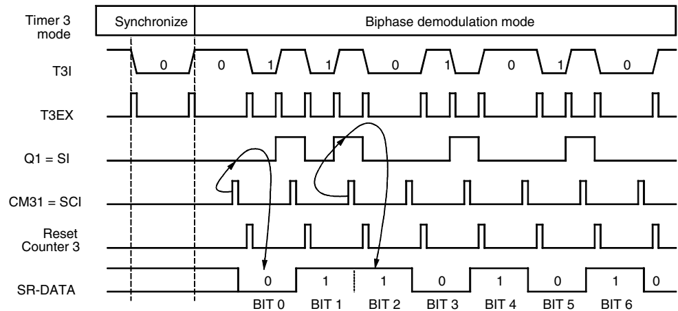
Figure 5-34. Timer 3 – Bi-phase Demodulation
