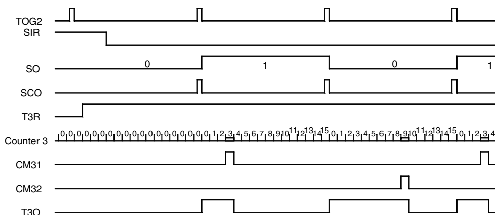
Figure 5-32. Pulse-width Modulation
