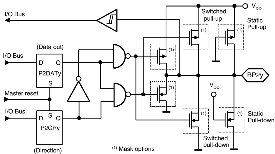
Figure 5-3. Bi-directional Port 2
