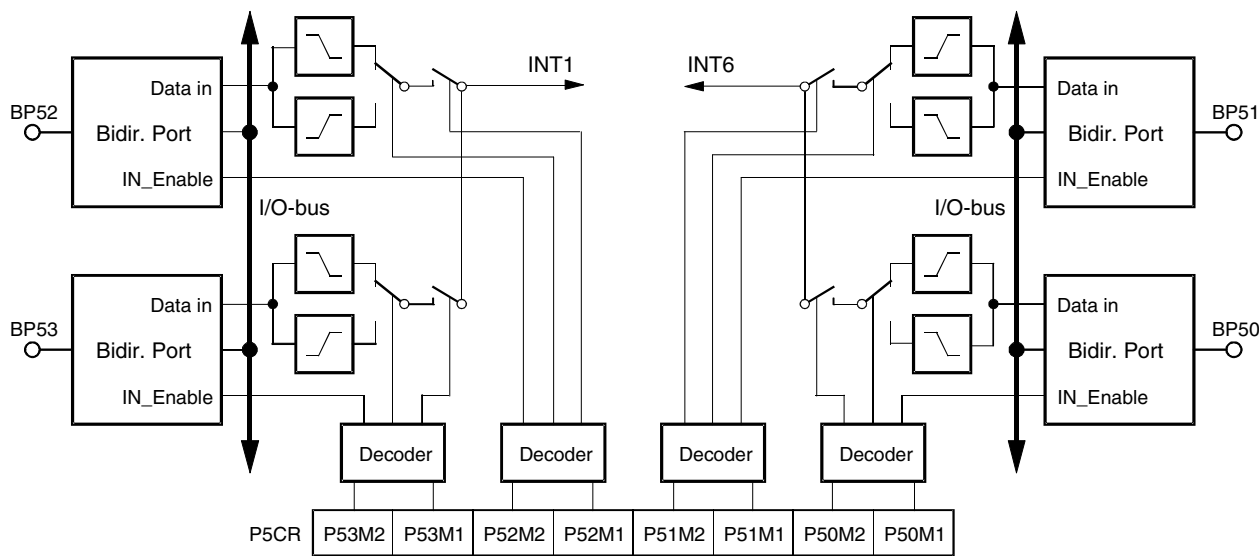
Figure 5-5. Port 5 External Interrupts
