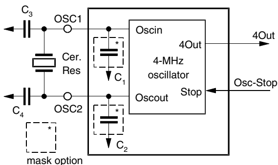
Figure 4-17. Ceramic Resonator
