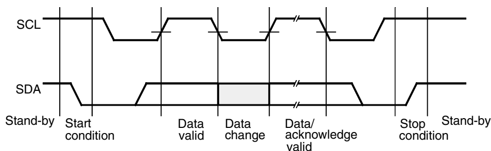
Figure 6-3. MCL Protocol
