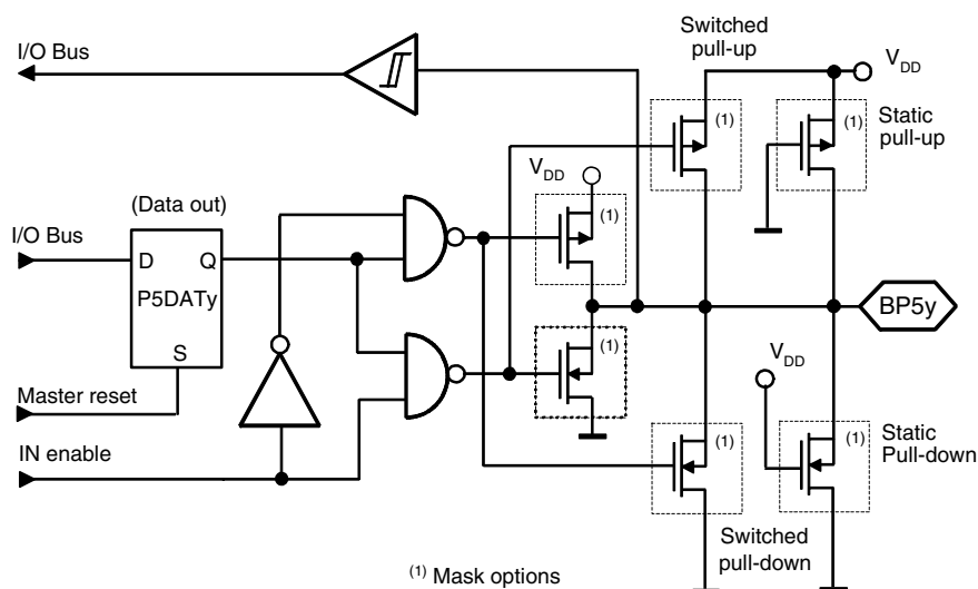
Figure 5-4. Bi-directional Port 5
