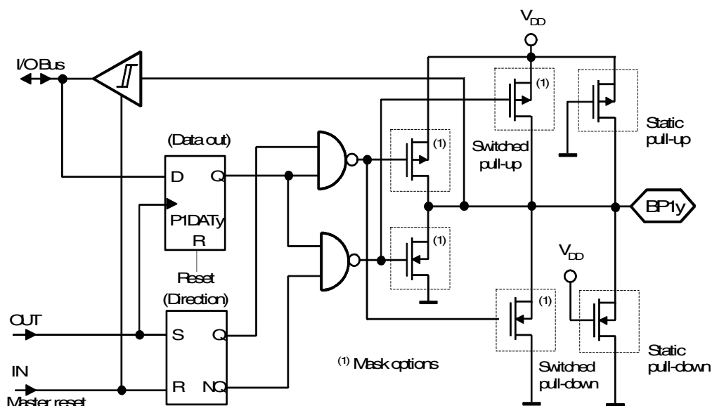
Figure 5-2. Bi-directional Port 1
