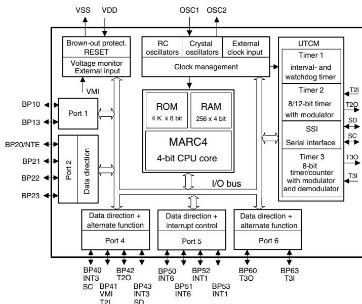
Figure 1-1. Block Diagram
