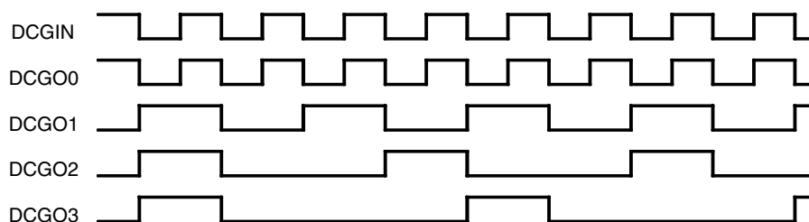
Figure 5-23. DCG Output Signals
