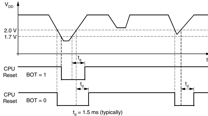
Figure 4-8. Brown-out Detection
