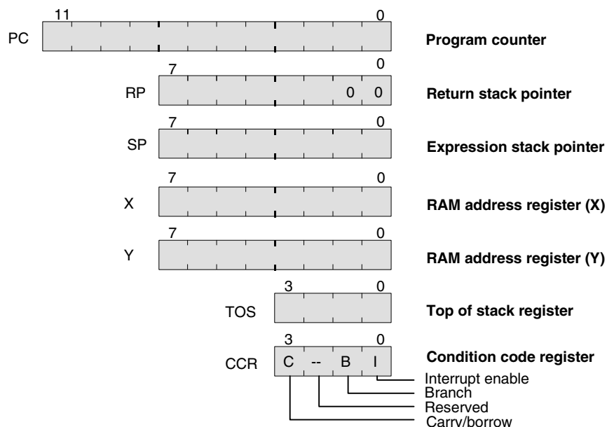
Figure 4-4. Programming Model
