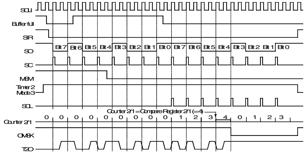
Figure 5-52. Manchester Modulation 2
