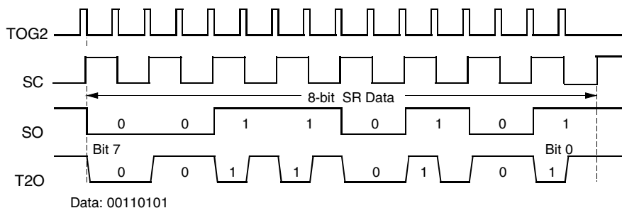
Figure 39. Bi-phase Modulation
