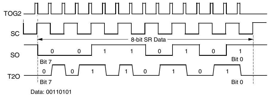
Figure 40. Manchester Modulation
