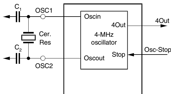
Figure 19. Ceramic Resonator
