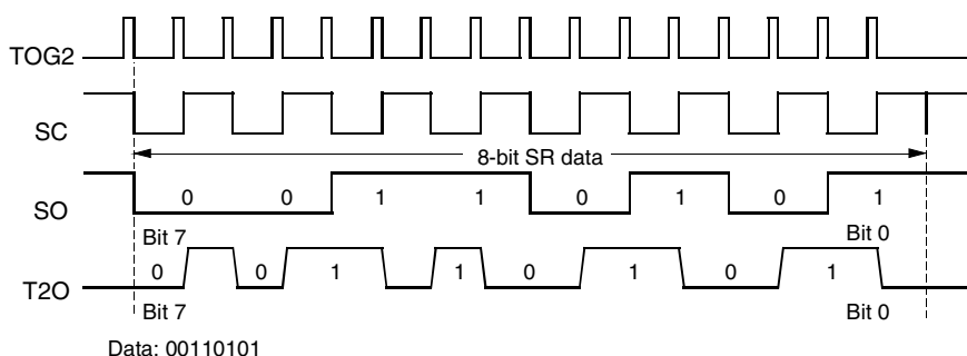
Figure 55. Manchester Modulation 1
