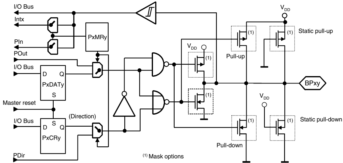
Figure 25. Bi-directional Port 4
