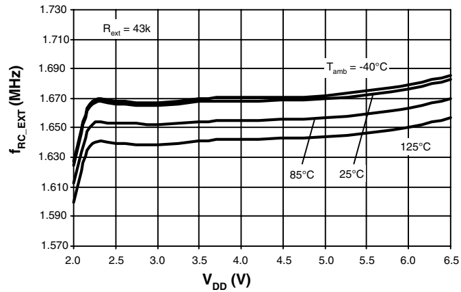
Figure 65. External RC Frequency versus V_{DD}
