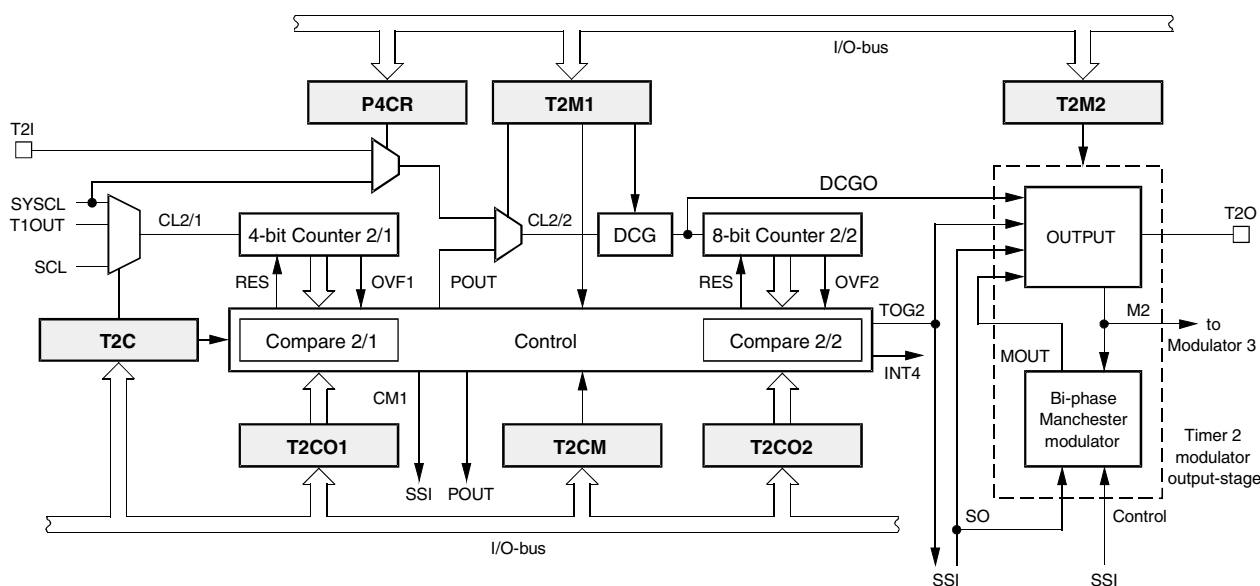
Figure 29. Timer 2
