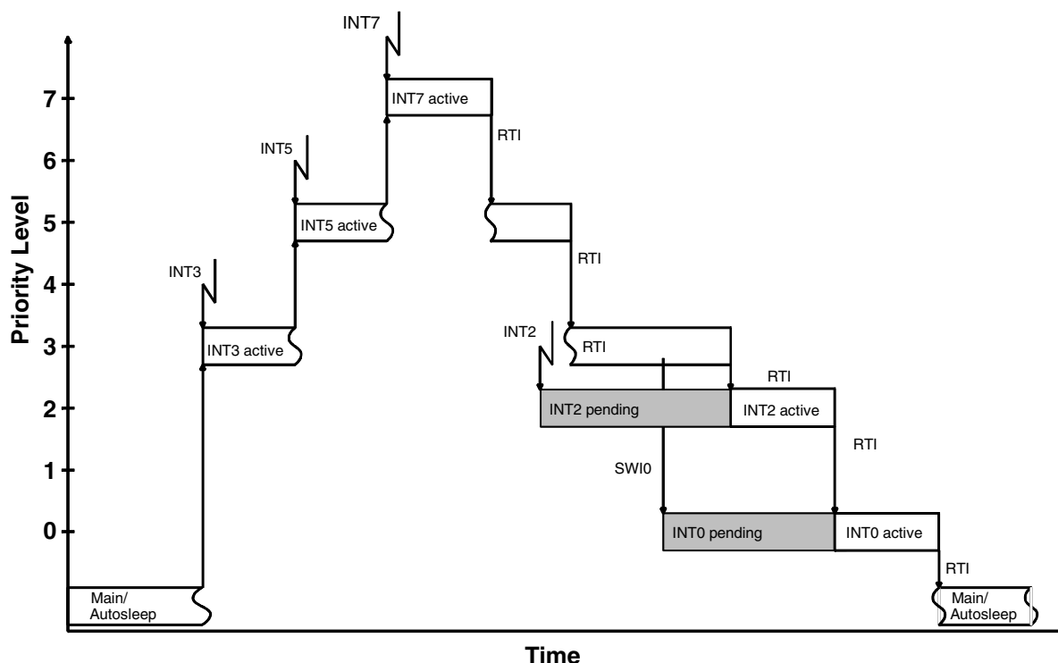
Figure 8. Interrupt Handling
