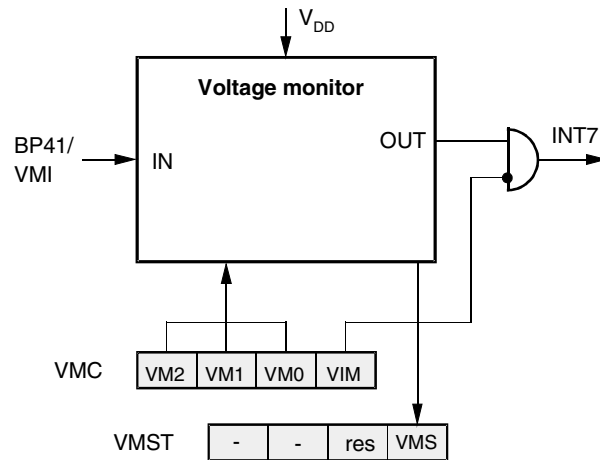
Figure 11. Voltage Monitor
