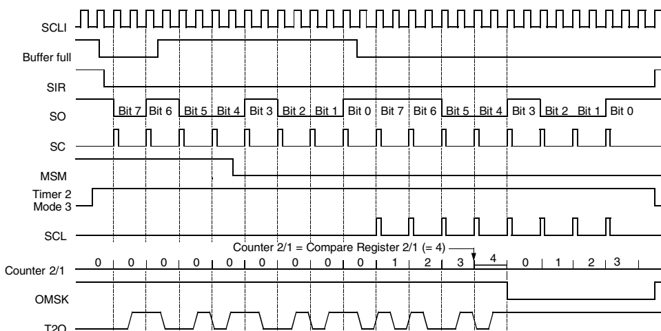
Figure 56. Manchester Modulation 2
