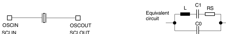
Figure 58. Crystal and Equivalent Circuit
