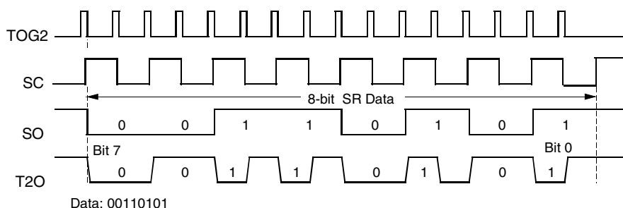
Figure 39. Bi-phase Modulation
