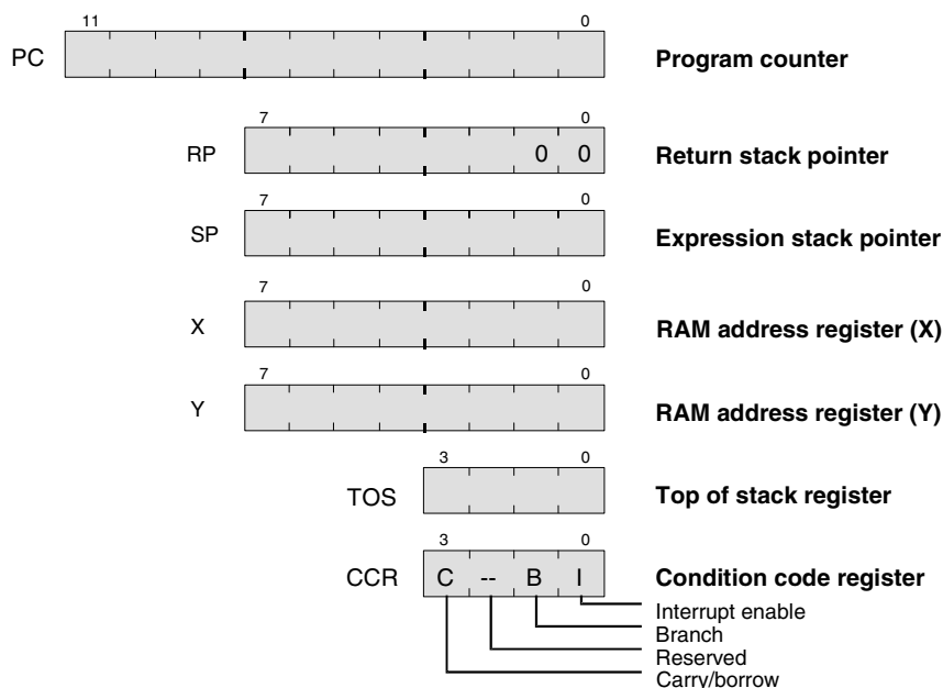
Figure 6. Programming Model
