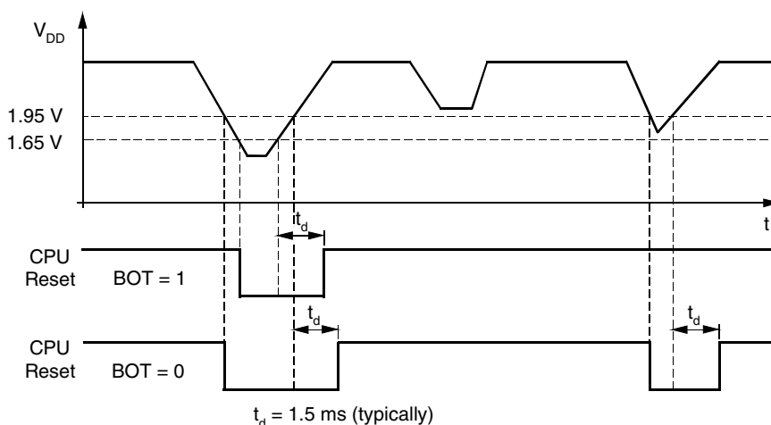
Figure 10. Brown-out Detection
