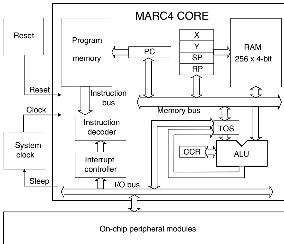
Figure 3. MARC4 Core
