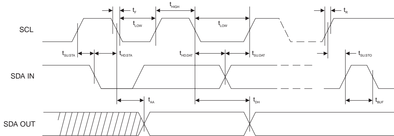
Figure 11-1. Bus Timing
