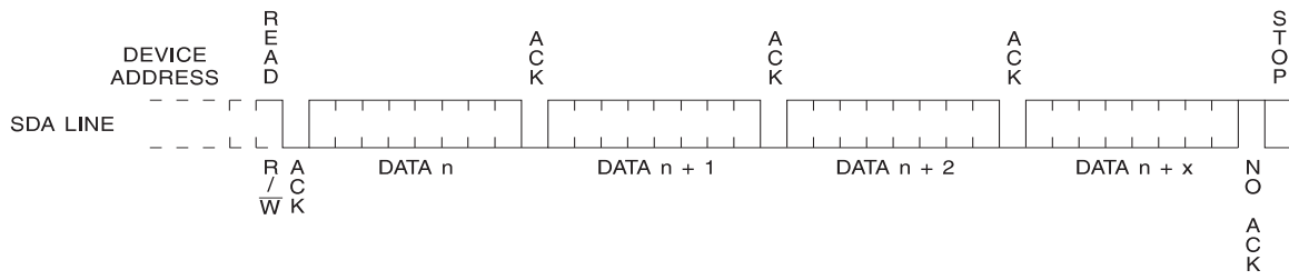
Figure 15. Sequential Read
