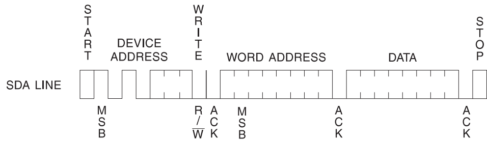
Figure 11. Byte Write
