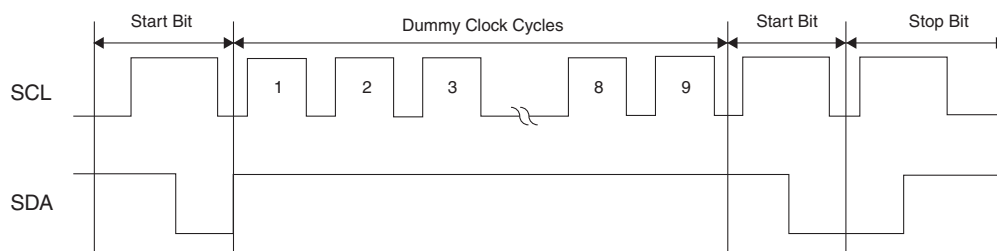
Figure 2. Bus Timing SCL: Serial Clock SDA: Serial Data I/O
