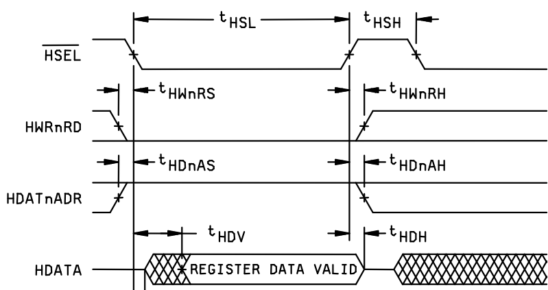
HOST READ DATA
