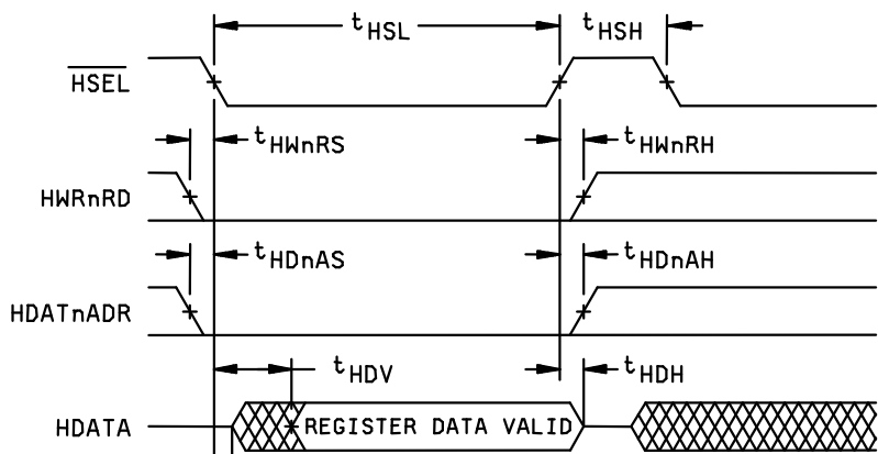
HOST READ ADDRESS
