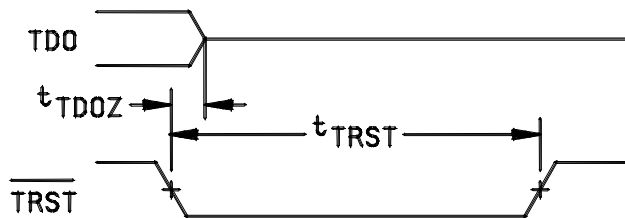
TEST PORT RESET
