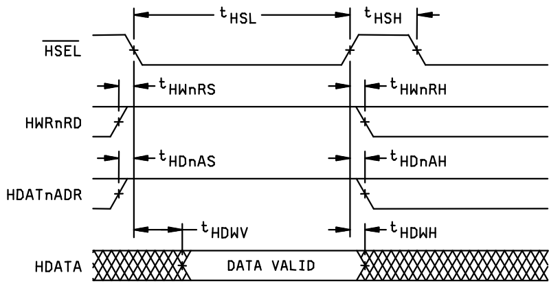
HOST WRITE DATA
