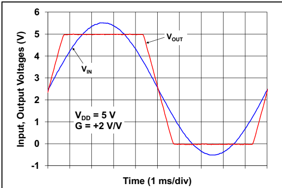
FIGURE 2-32: The MCP6481 Shows No Phase Reversal.
