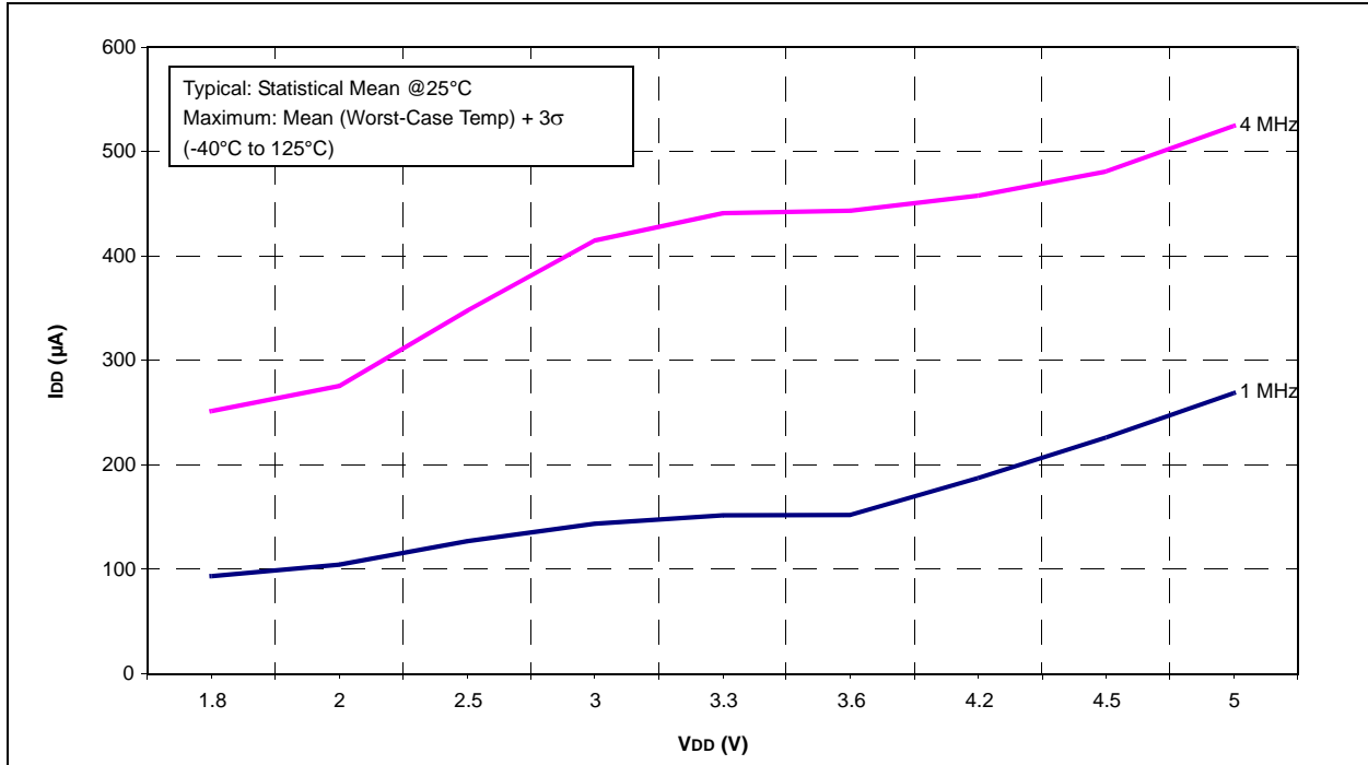
FIGURE 26-5: PIC16F707 MAXIMUM I DD vs. V DD OVER F OSC , EXTRC MODE, V CAP = 0.1μF
