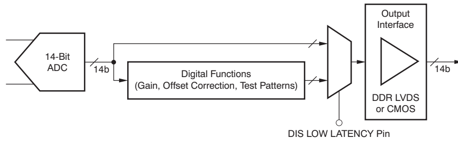
Figure 122. Digital Processing Block Diagram
