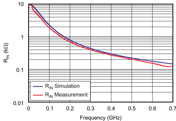
Figure 60. ADC Analog Input Resistance ( R_{IN} ) Across Frequency
