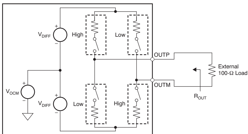
Figure 57. LVDS Buffer Equivalent Circuit
