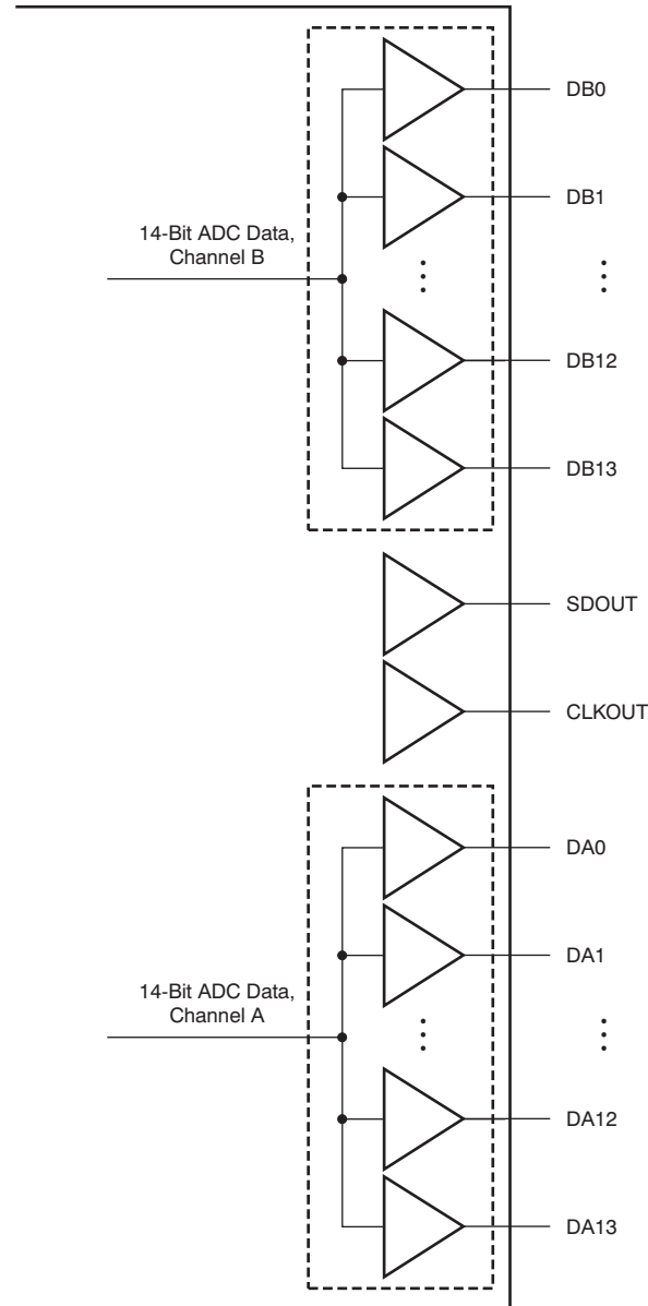
Figure 59. CMOS Outputs
