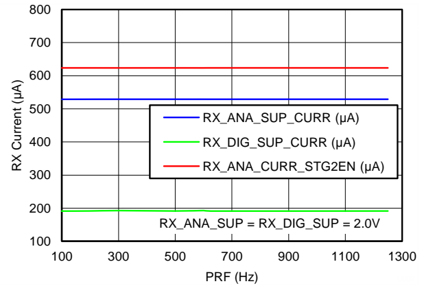
Figure 4. TOTAL Rx CURRENT vs PRF
