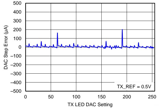
Figure 34. TRANSMITTER DAC CURRENT STEP ERROR (150 mA, Max)
