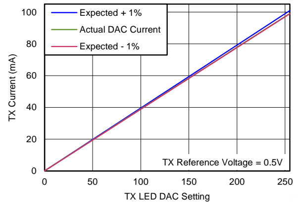
Figure 40. TRANSMITTER CURRENT LINEARITY (100-mA Range)
