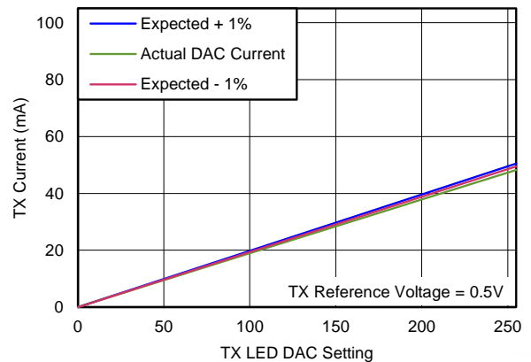
Figure 38. TRANSMITTER CURRENT LINEARITY (50-mA Range)
