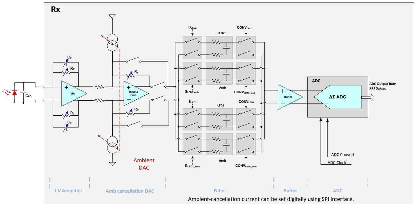
Figure 54. Receiver Front-End
