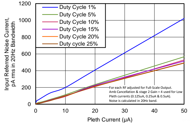
Figure 16. INPUT-REFERRED NOISE CURRENT vs PLETH CURRENT (BW = 20 Hz, PRF = 1200 Hz)
