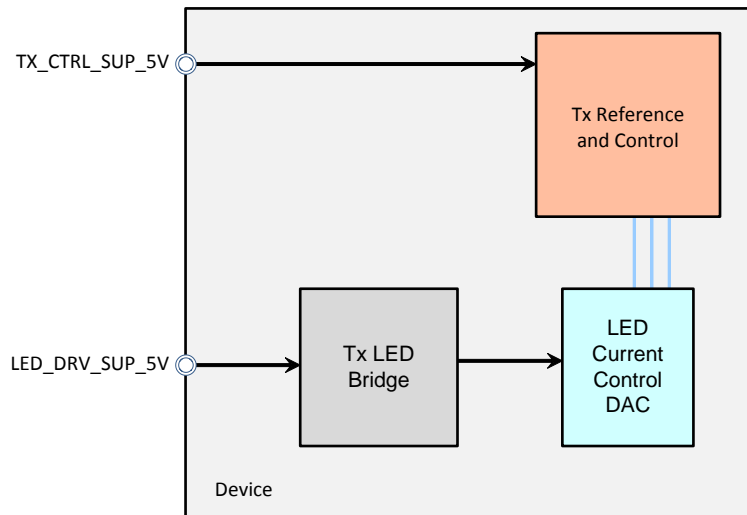
Figure 73. Transmit Subsystem Power Routing
