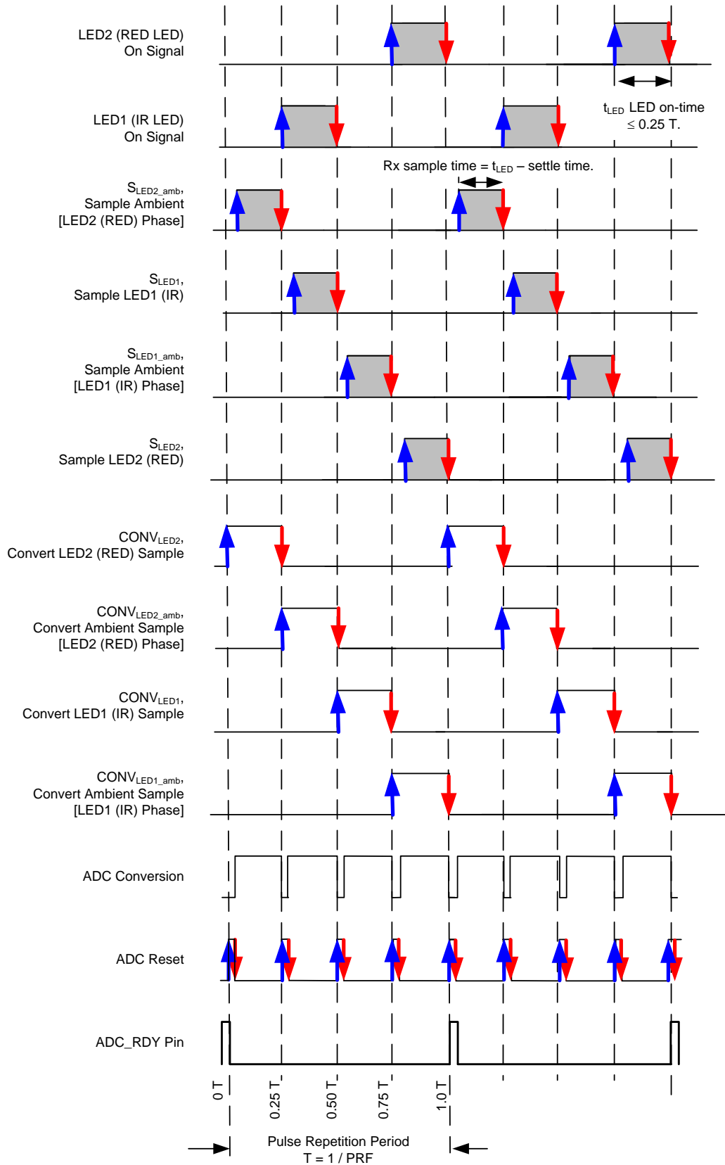
Figure 59. AFE Control Signals
