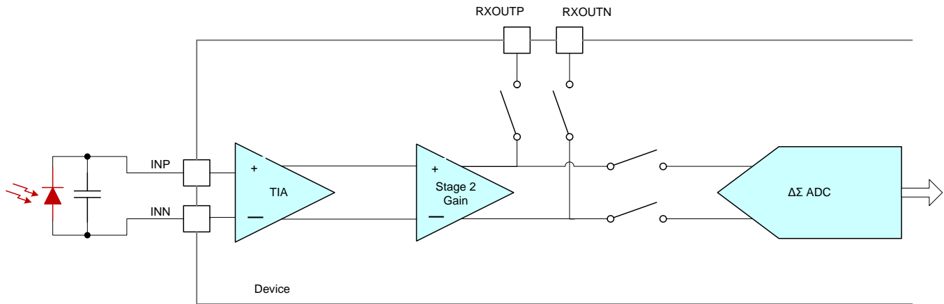
Figure 67. AFE4490 Set to ADC Bypass Mode
