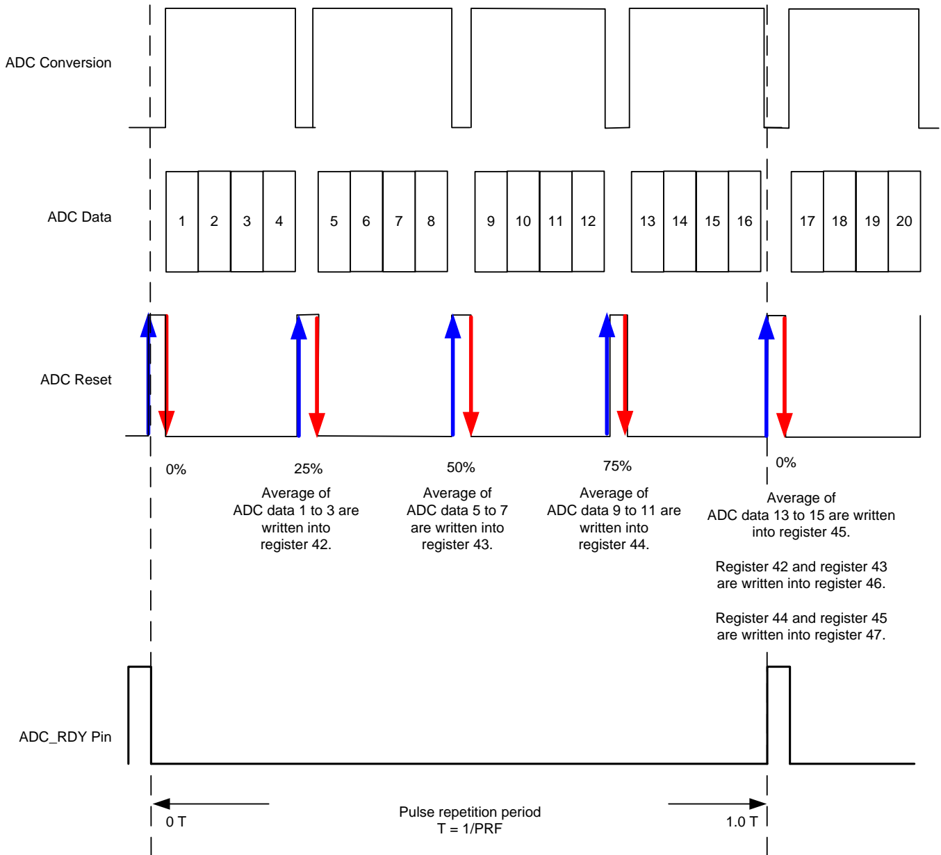
Figure 66. ADC Data with Averaging Enabled
