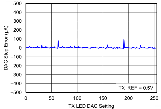
Figure 36. TRANSMITTER DAC CURRENT STEP ERROR (75 mA, Max)
