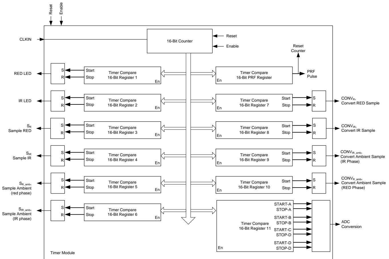
Figure 61. Timer Module
