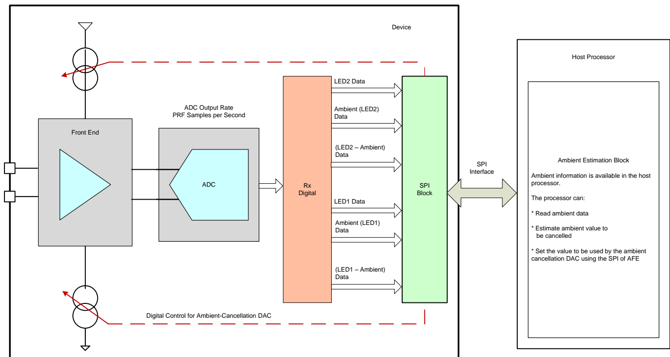
Figure 55. Ambient Cancellation Loop (Closed by the Host Processor)
