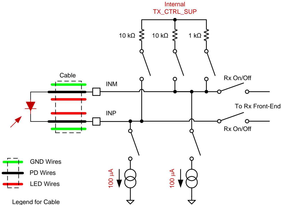
Figure 75. Photodiode Diagnostic
