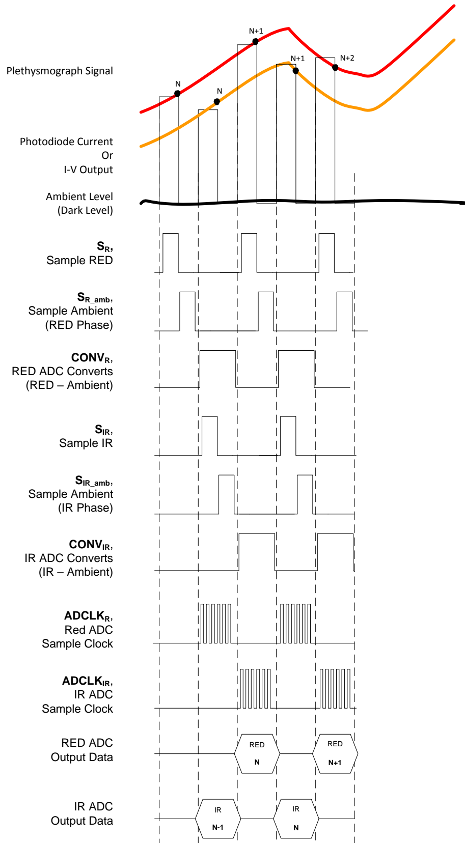
Figure 57. Rx Timing Diagram
