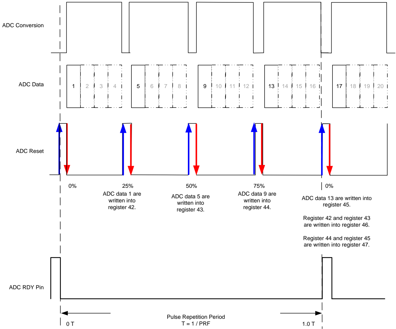
Figure 65. ADC Data Without Averaging (When Number of Averages = 0)
