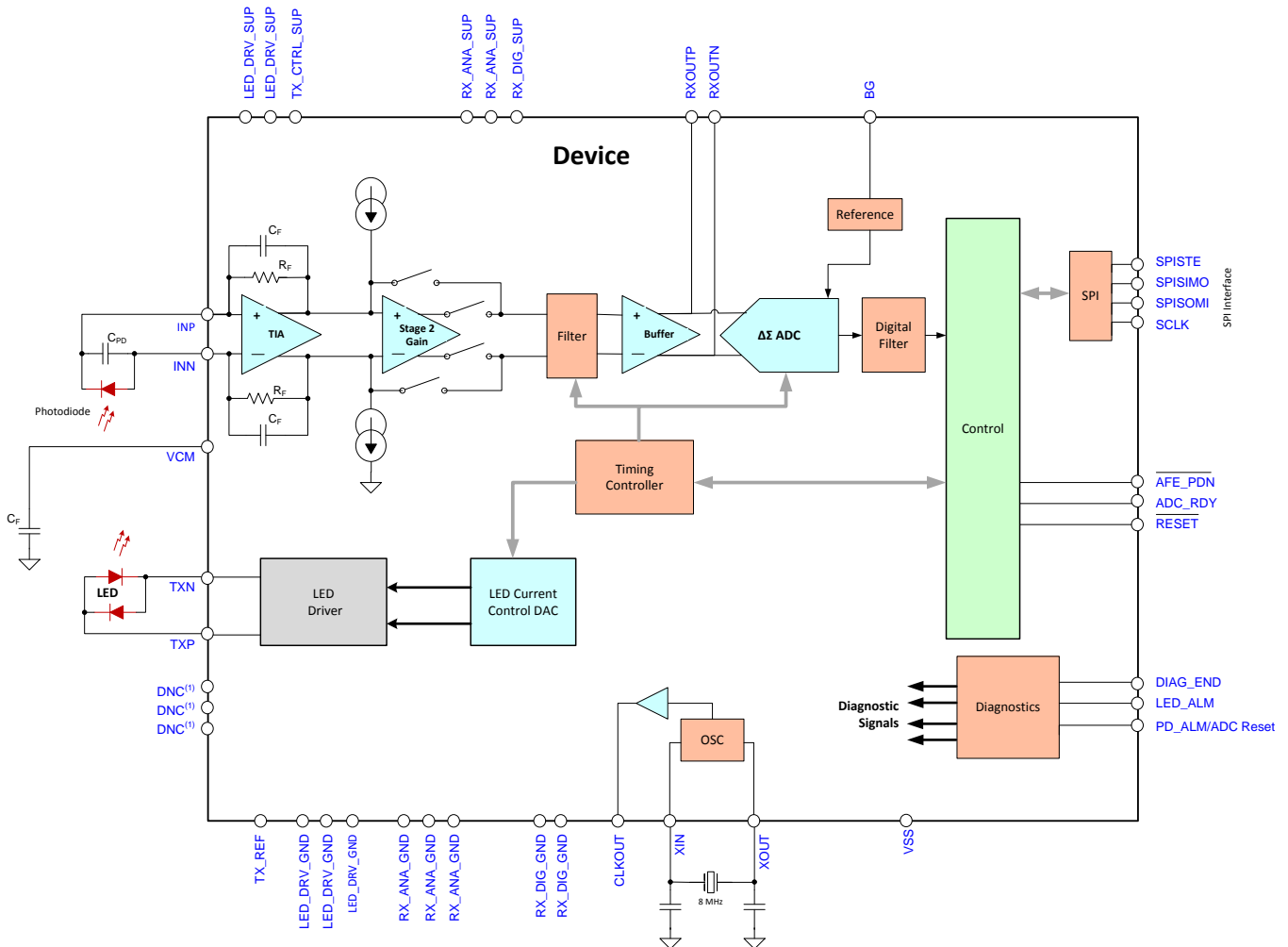
Figure 53. Detailed Block Diagram
