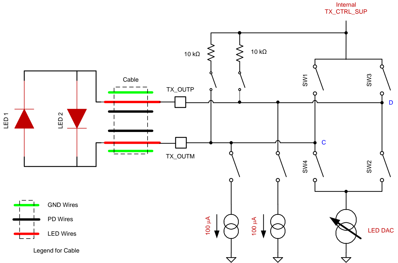
Figure 76. Transmitter Diagnostic
