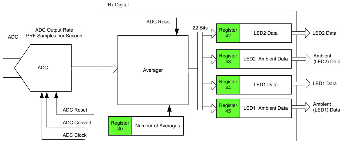
Figure 64. Averaging Module
