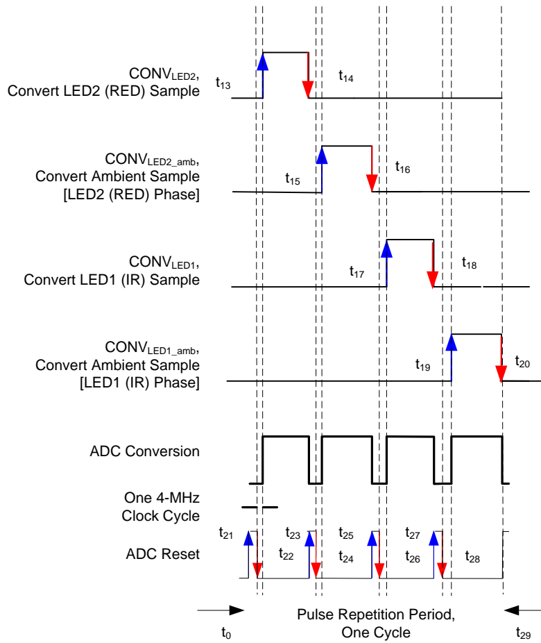
Figure 63. Relationship Between the ADC Reset and ADC Conversion Signals
