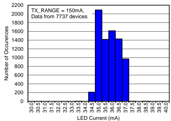
Figure 44. LED CURRENT WITH Tx DAC SETTING = 60 (35 mA)
