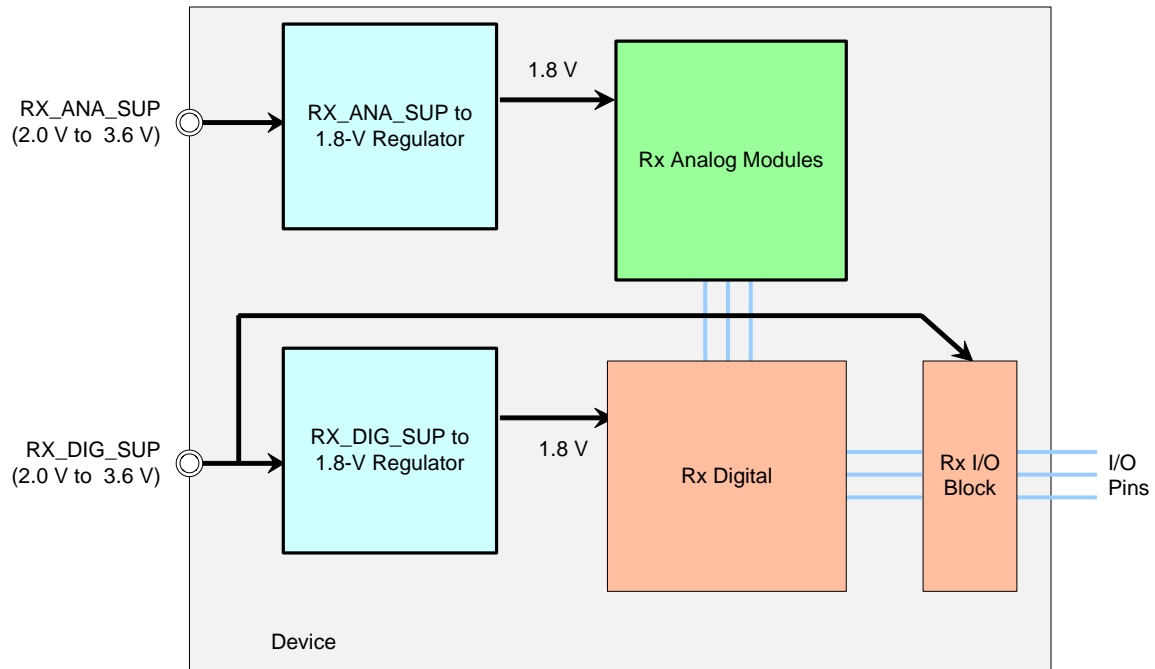
Figure 70. Receive Subsystem Power Routing
