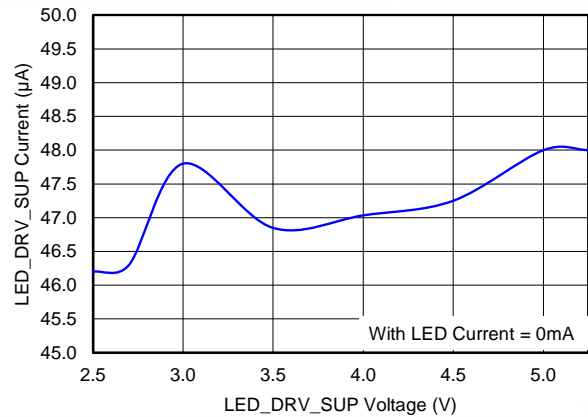
Figure 6. LED_DRV_SUP CURRENT vs LED_DRV_SUP VOLTAGE
