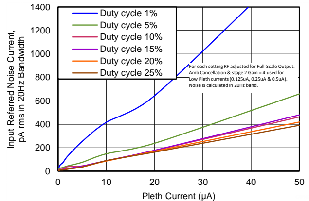
Figure 18. INPUT-REFERRED NOISE CURRENT vs PLETH CURRENT (BW = 20 Hz, PRF = 5000 Hz)
