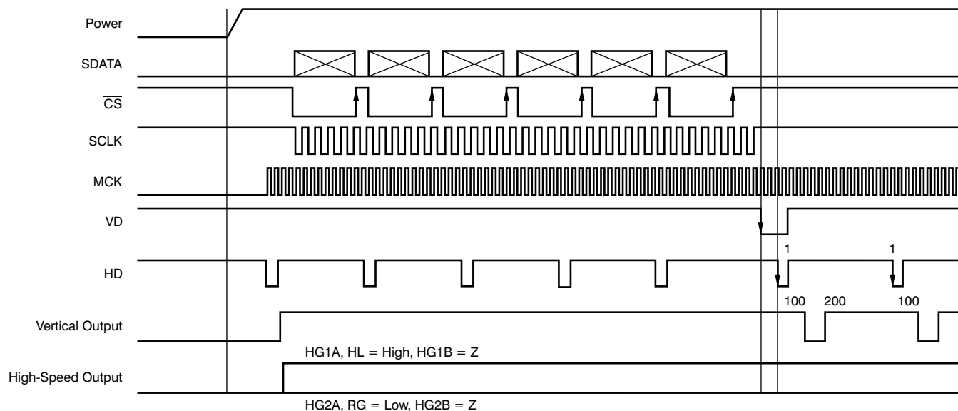
Figure 17. Power-Up Sequence
