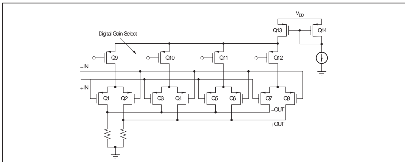
Figure 55. Programmable LNP
