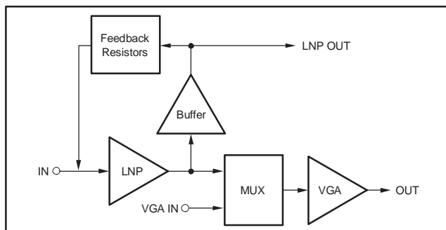
Figure 56. Block Diagram of LNP/VGA Interface
