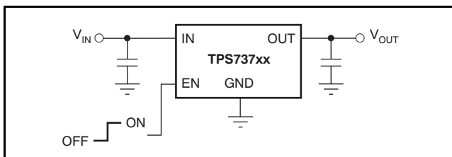
Figure 31. Typical Application Circuit for Fixed-Voltage Version
