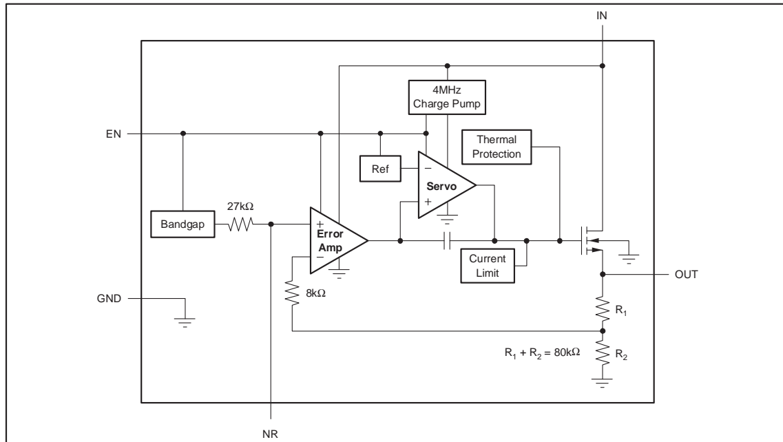
Figure 2. Fixed Voltage Version
