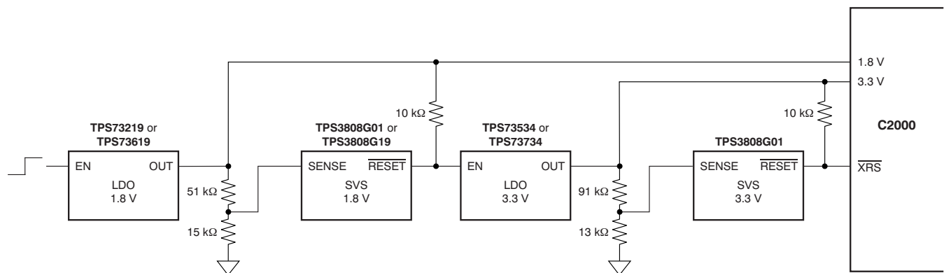
Figure 1. Typical Application
