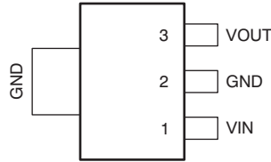
DCY PACKAGE SOT223 (TOP VIEW)
