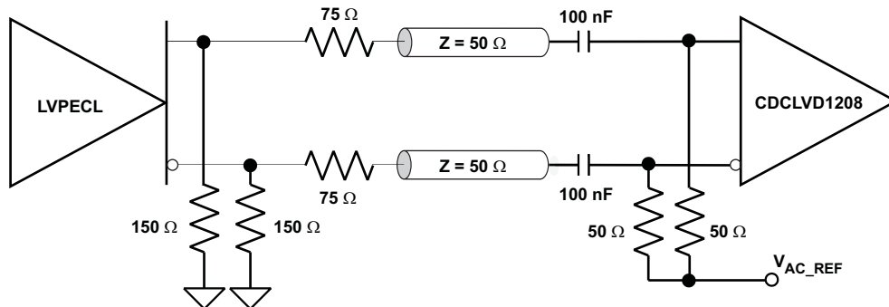
Figure 18. LVPECL Clock Driver Connected to CDCLVD1208 Input
