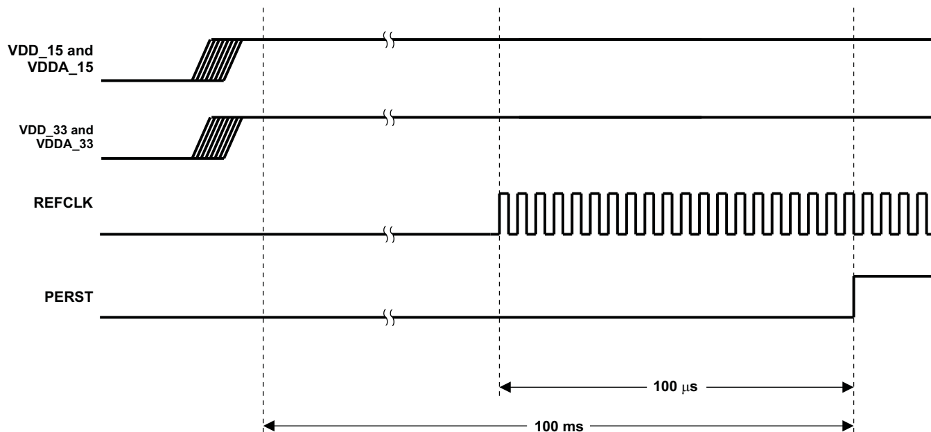
Figure 3-2. Power-Up Sequence
