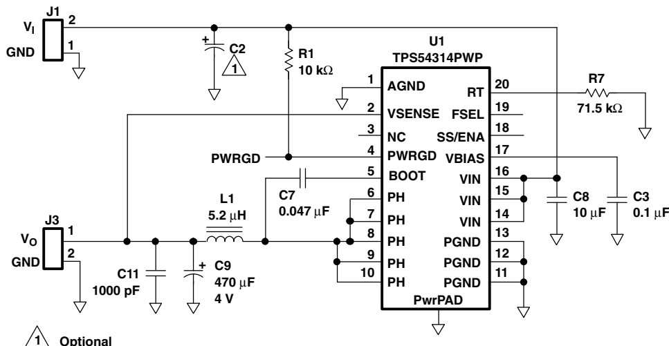
Figure 10. TPS54314 Schematic
