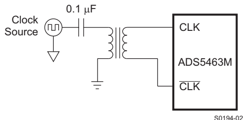
Figure 19. Differential Clock
