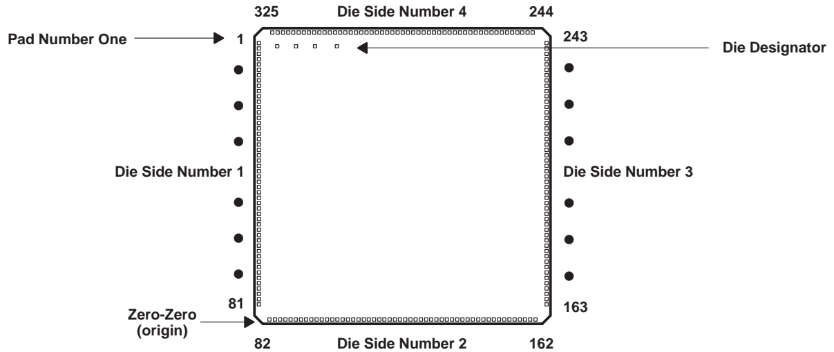
Figure 2. 320C40 Die Numbering Format (See Table 1)
