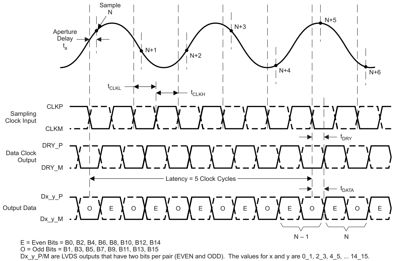
Figure 1. Timing Diagram
