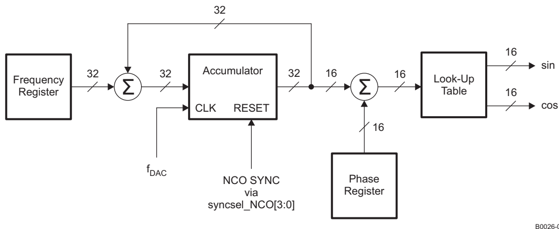
Figure 72. NCO Block Diagram
