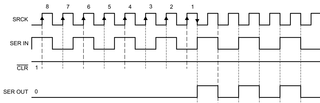
Figure 8. SER IN to SER OUT Waveform
