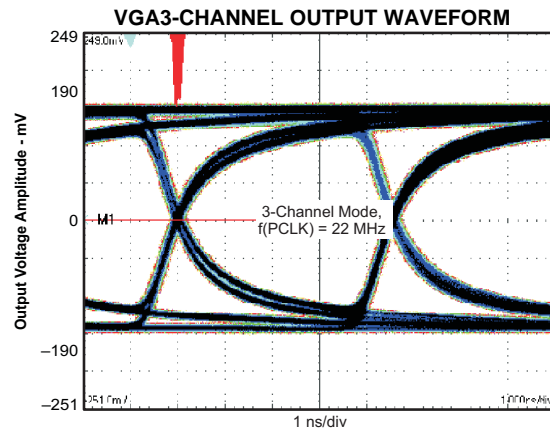
Response Over 80-inch FR-4 + 1m Coax Cable
