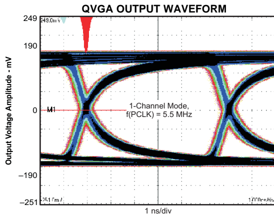
Response Over 80-inch of FR-4 + 1m Coax Cable
