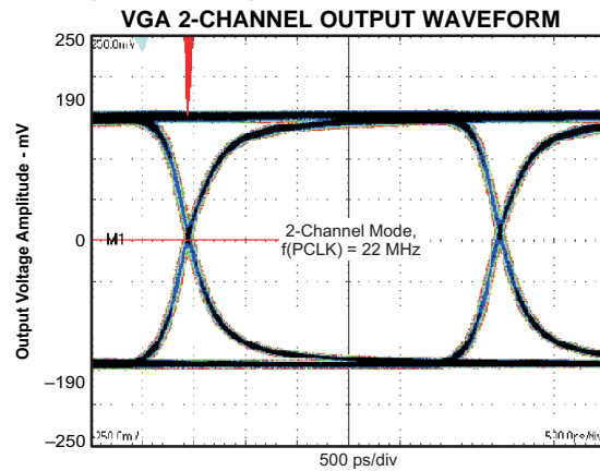
Response Over 8-inch FR-4 + 1m Coax Cable
