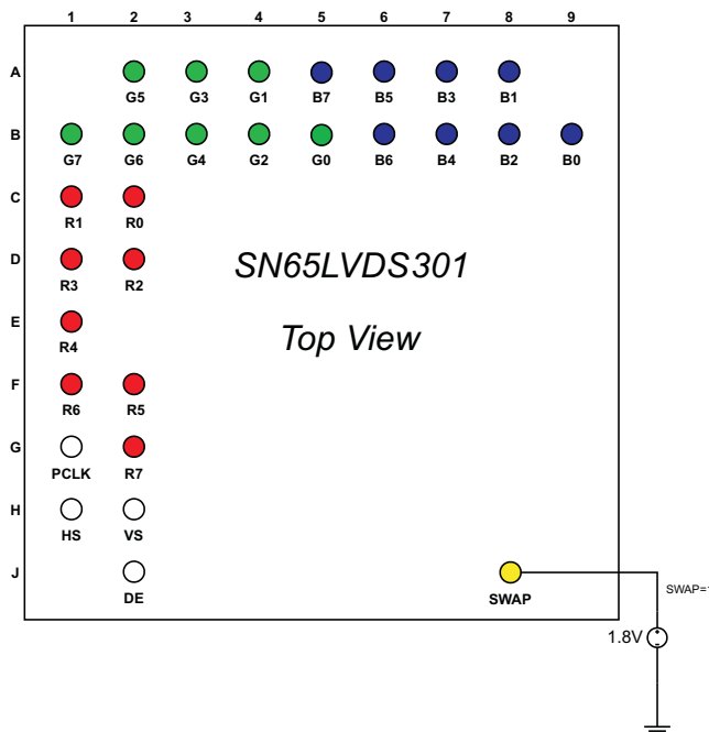
Figure 2. SWAP PIN = 1
