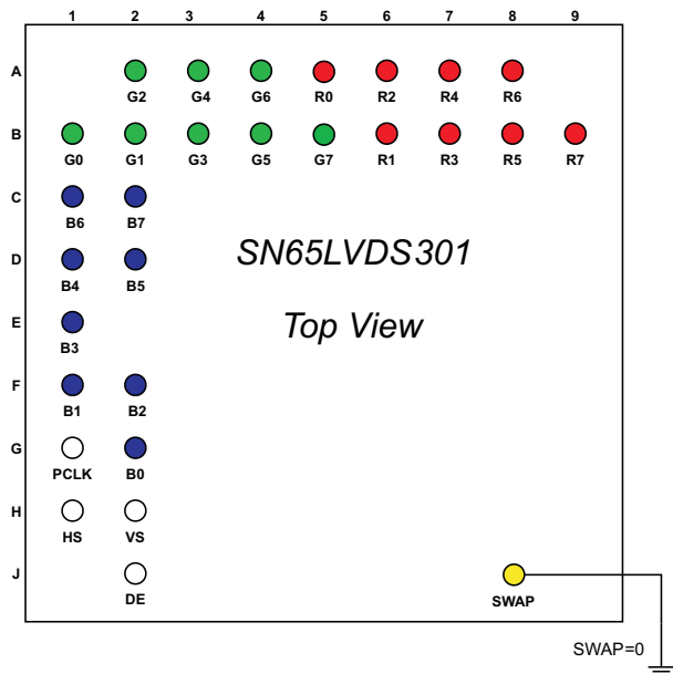
Figure 1. SWAP PIN = 0
