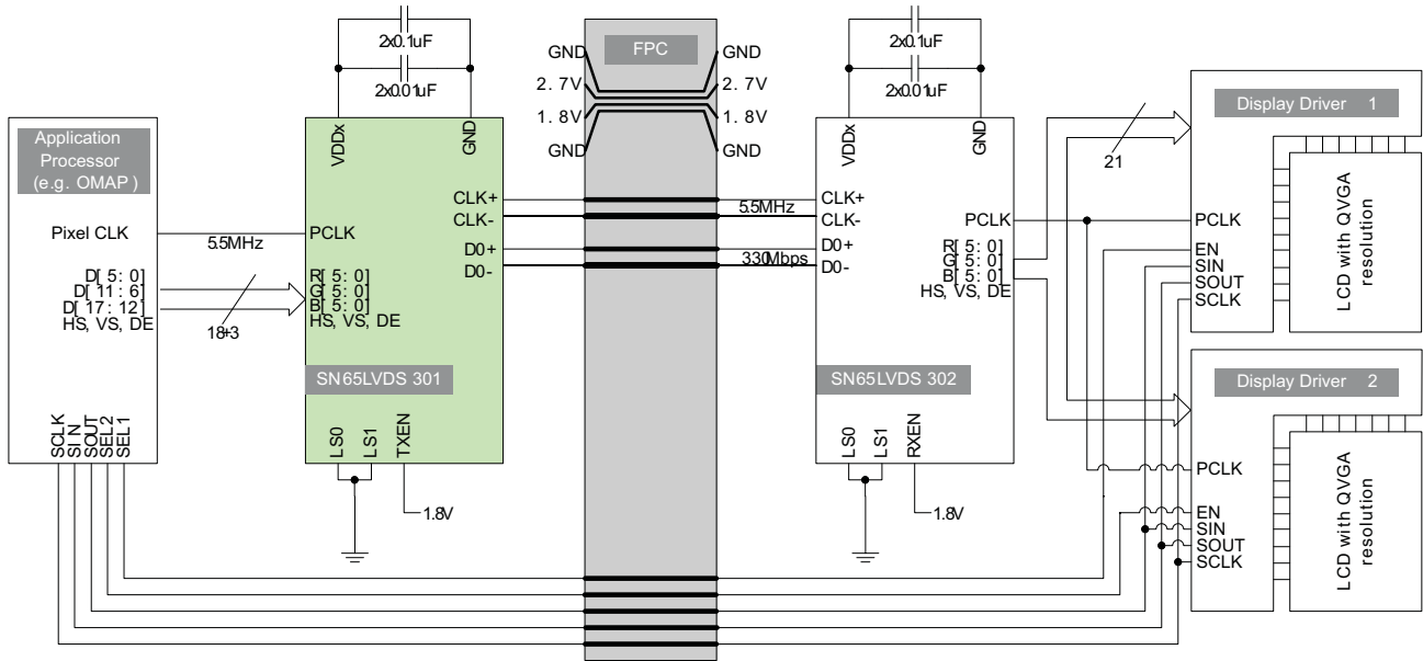
Figure 41. Example Dual-QVGA Display Application
