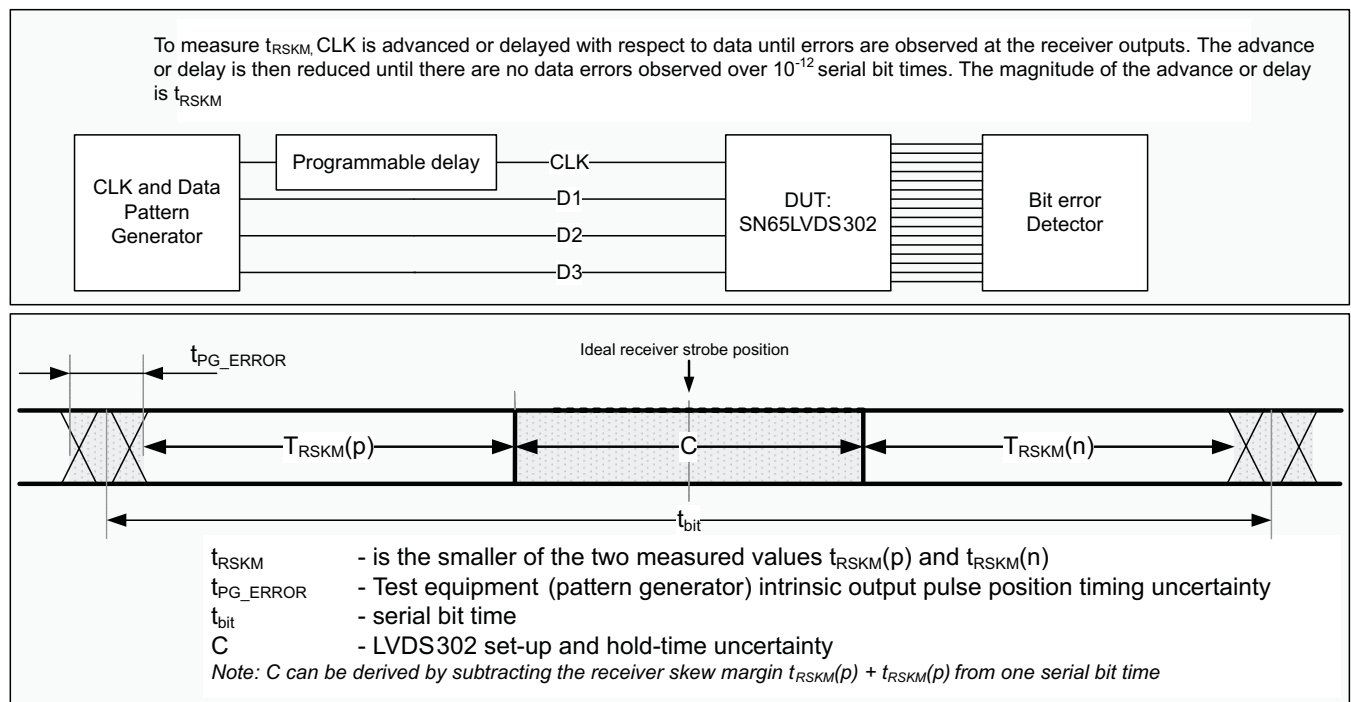
Figure 8. Jitter Budget
