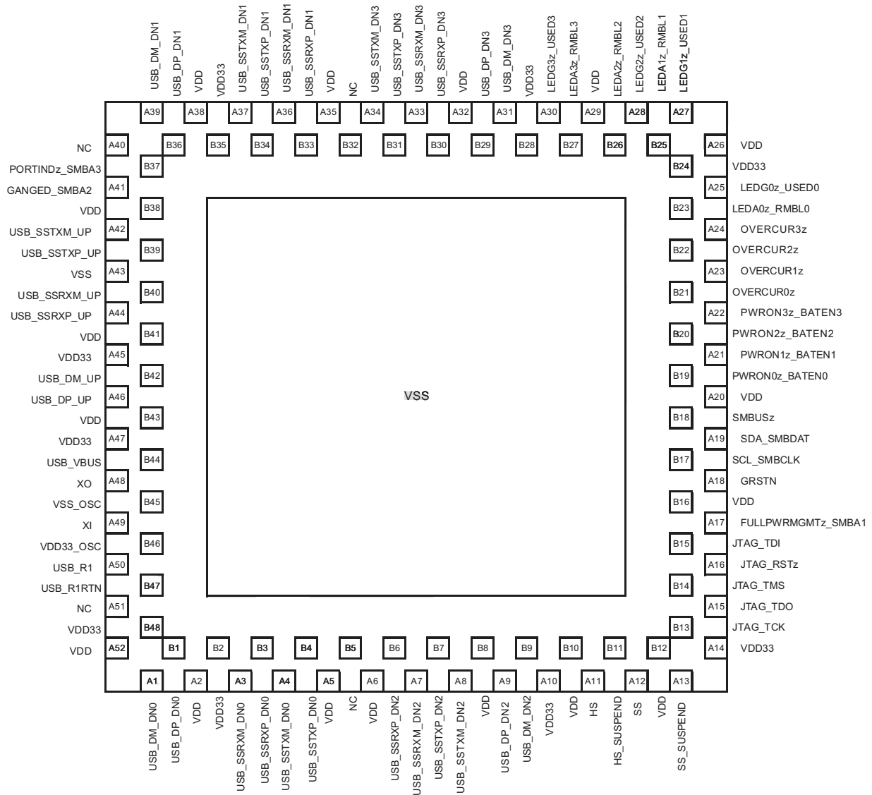
TUSB8040A1RKM (Top View)
