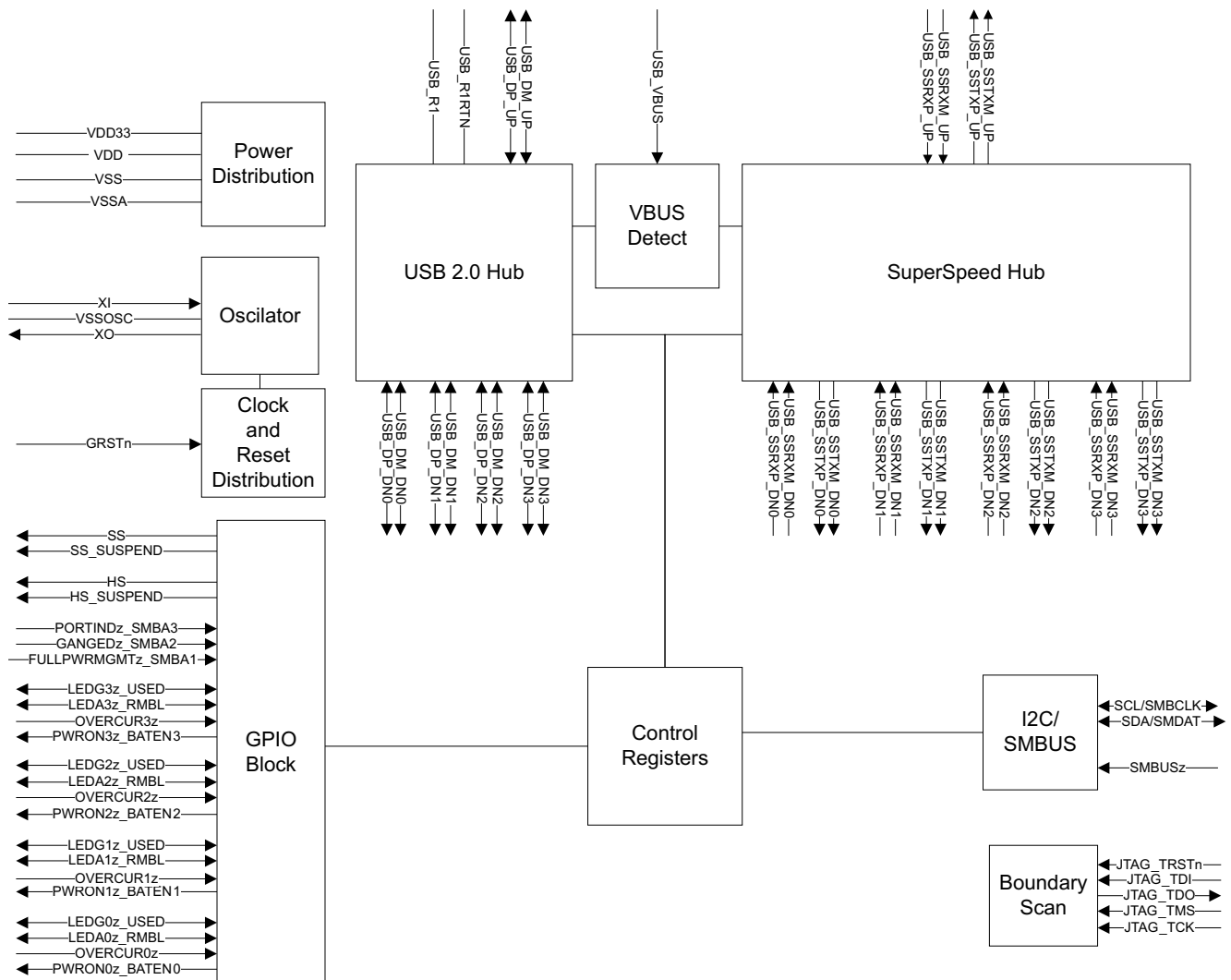
Figure 1-2. TUSB8040A1 Functional Block Diagram
