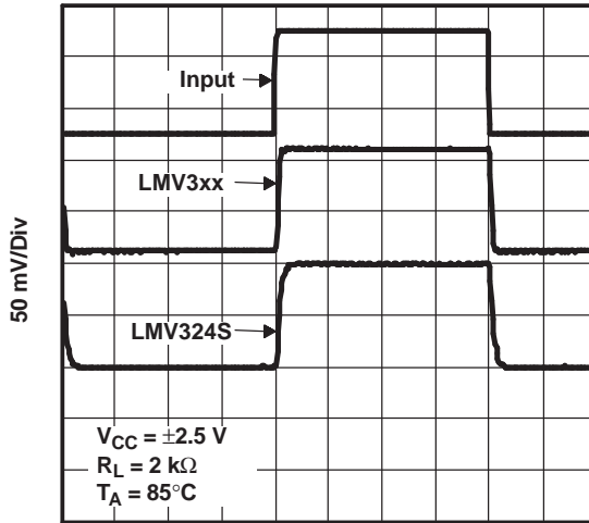
1 \mu\text{s}/\text{Div} Figure 31.
