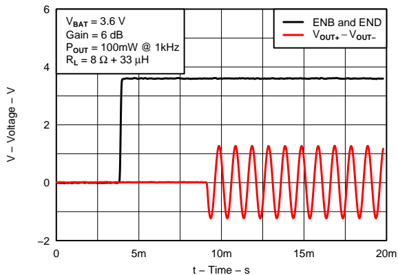
Figure 15. STARTUP TIMING
