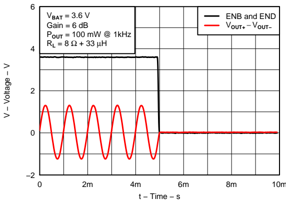
Figure 16. SHUTDOWN TIMING
