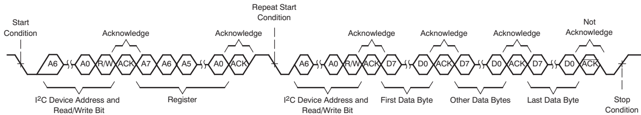
Figure 44. Multiple-Byte Read Transfer
