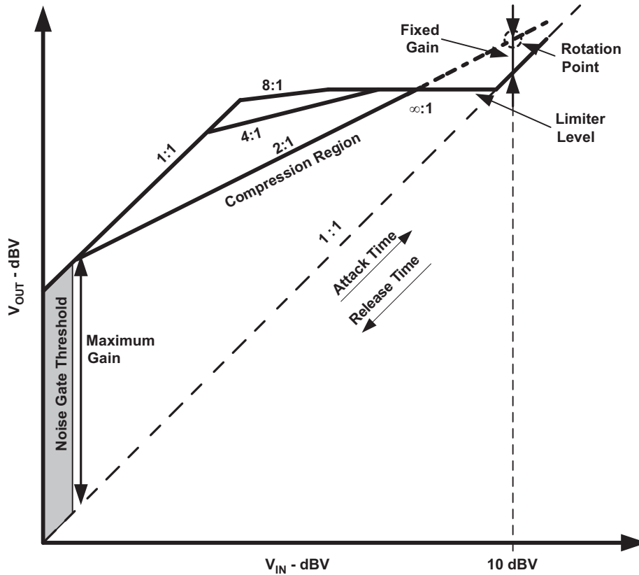
Figure 39. Output Signal vs. Input Signal State Diagram
