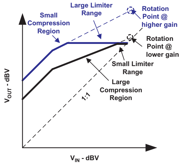
Figure 35. Output Signal vs Input Signal State Diagram Showing the Effects of the Limiter Range to the Compression Region
