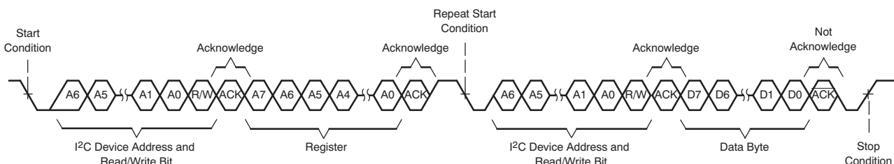
Figure 43. Single-Byte Read Transfer
