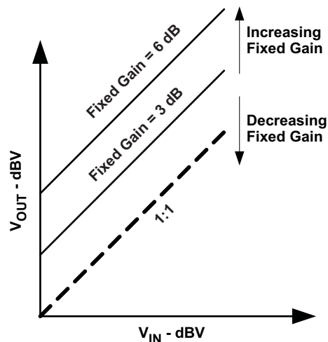
Figure 31. Output Signal vs Input Signal State Diagram Showing Different Fixed Gain Configurations
