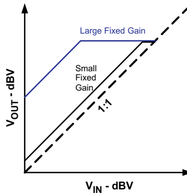
Figure 33. Output Signal vs. Input Signal State Diagram Showing Same Limiter Level Configurations with Different Fixed Gain Configurations
