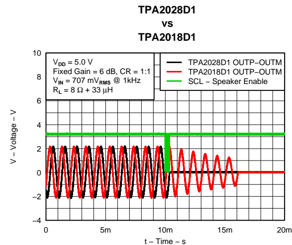
Figure 25. Shutdown Gain Ramp Comparison
