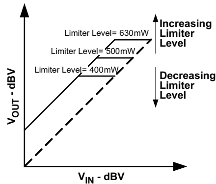
Figure 32. Output Signal vs Input Signal State Diagram Showing Different Limiter Level Configurations
