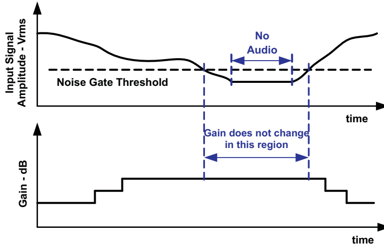
Figure 36. Time Diagram Showing the Relationship Between Input Signal Amplitude, Noise Gate Threshold and Gain Versus Time
