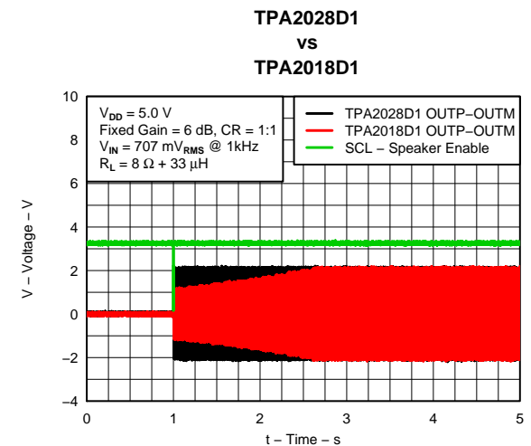
Figure 26. Startup Gain Ramp Comparison
