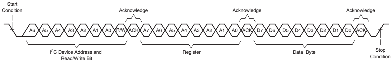
Figure 41. Single-Byte Write Transfer
