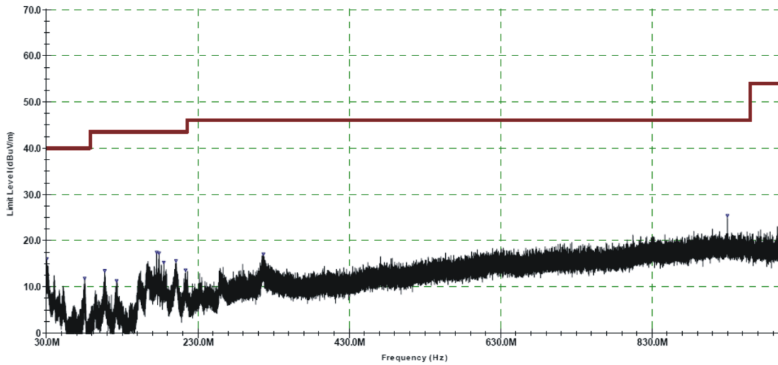
Figure 47. EMC Performance under FCC Class-B
