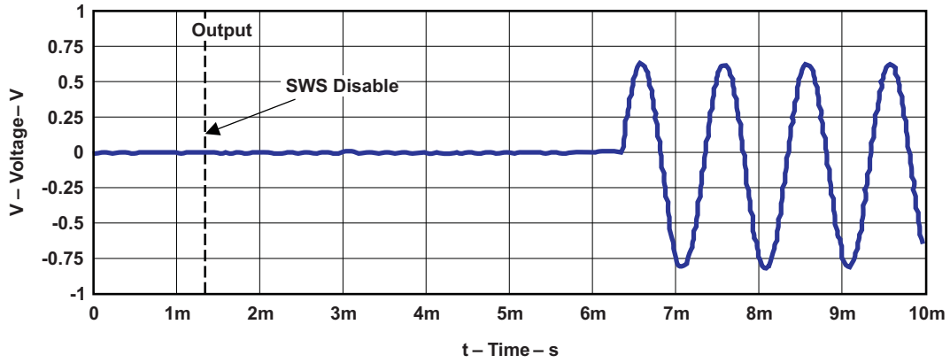
Figure 27. Startup Time
