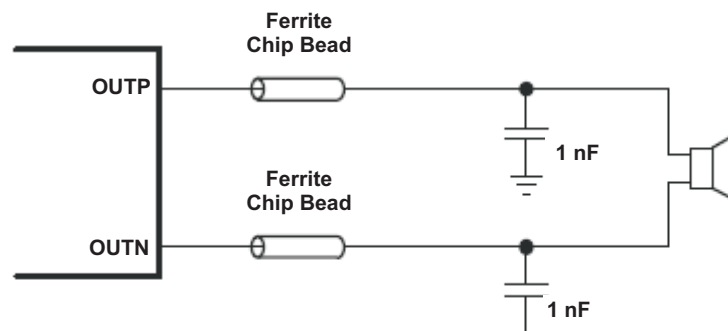
Figure 46. Typical Ferrite Bead Filter (Chip bead example: TDK: MPZ1608S221A)
