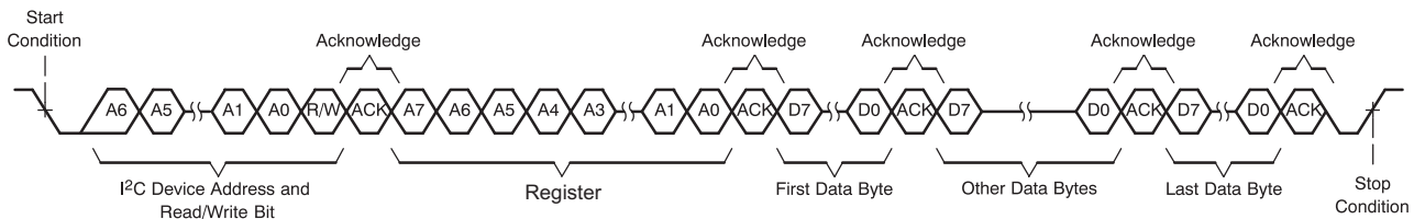
Figure 42. Multiple-Byte Write Transfer
