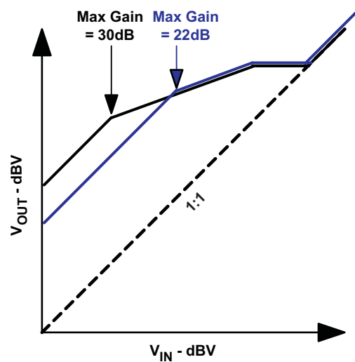
Figure 37. Output Signal vs. Input Signal State Diagram Showing Different Maximum Gains
