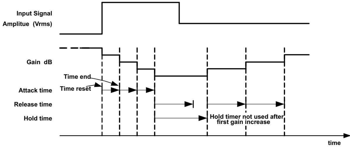
Figure 38. Time Diagram Showing the Relation Between the Attack, Release, and Hold Time vs Input Signal Amplitude and Gain
