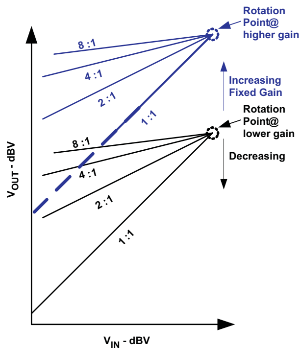
Figure 34. Output Signal vs Input Signal State Diagram Showing Different Compression Ratio Configurations with Different Fixed Gain Configurations
