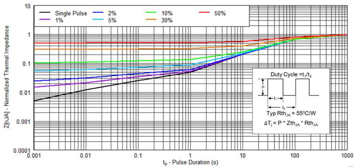
Figure 1. Transient Thermal Impedance
