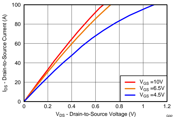
Figure 3. Saturation Characteristics
