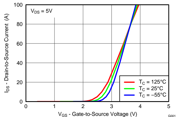
Figure 4. Transfer Characteristics
