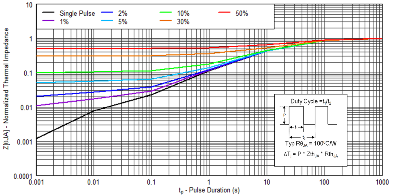
Figure 2. Transient Thermal Impedance
