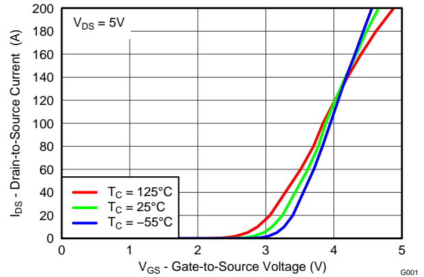
Figure 4. Transfer Characteristics
