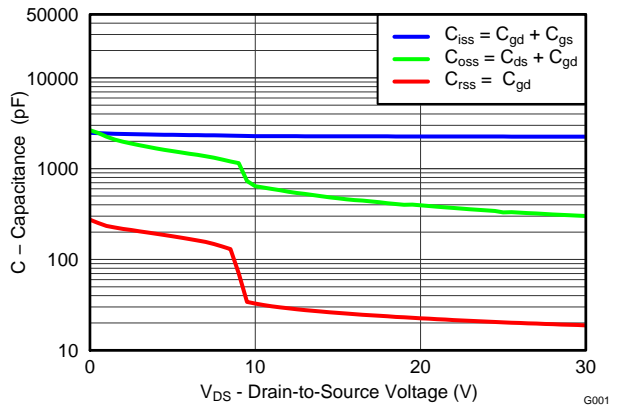
Figure 6. Capacitance
