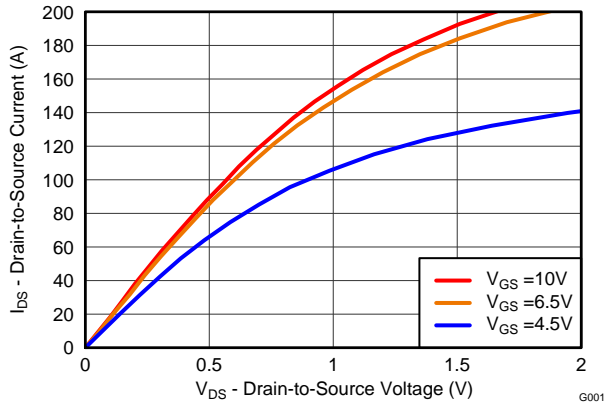
Figure 3. Saturation Characteristics
