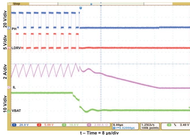
Figure 12. Battery-to-GND Short Transition
