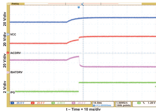
Figure 14. Input ACOV Transition
