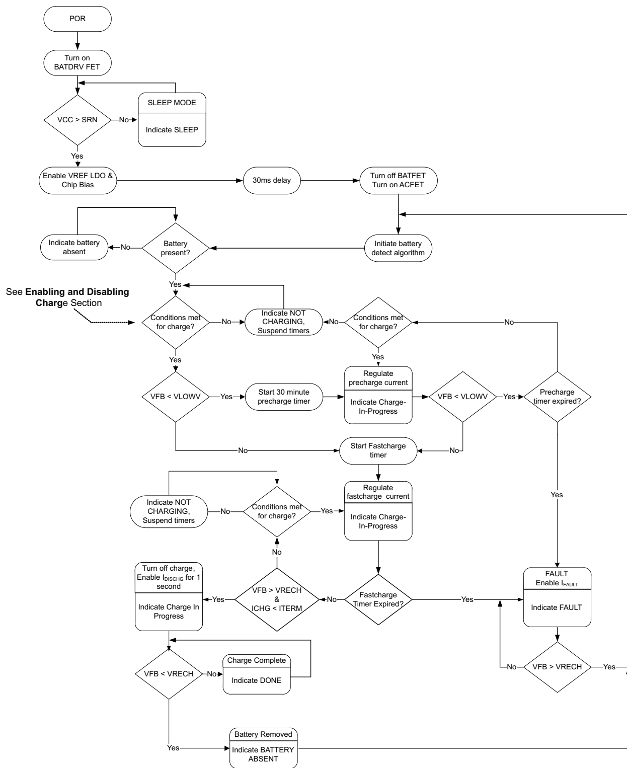
Figure 16. Operational Flowchart
